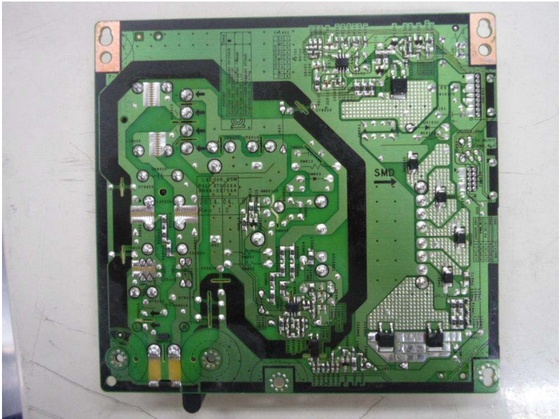
(Power Board)
