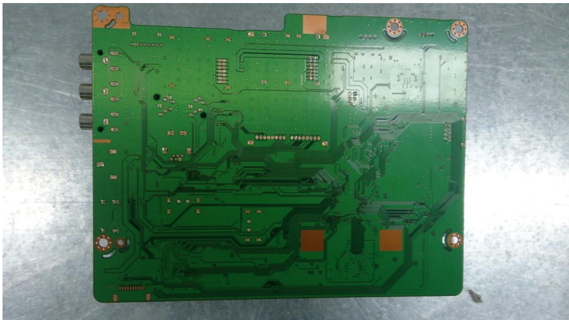
(MAIN Board )
