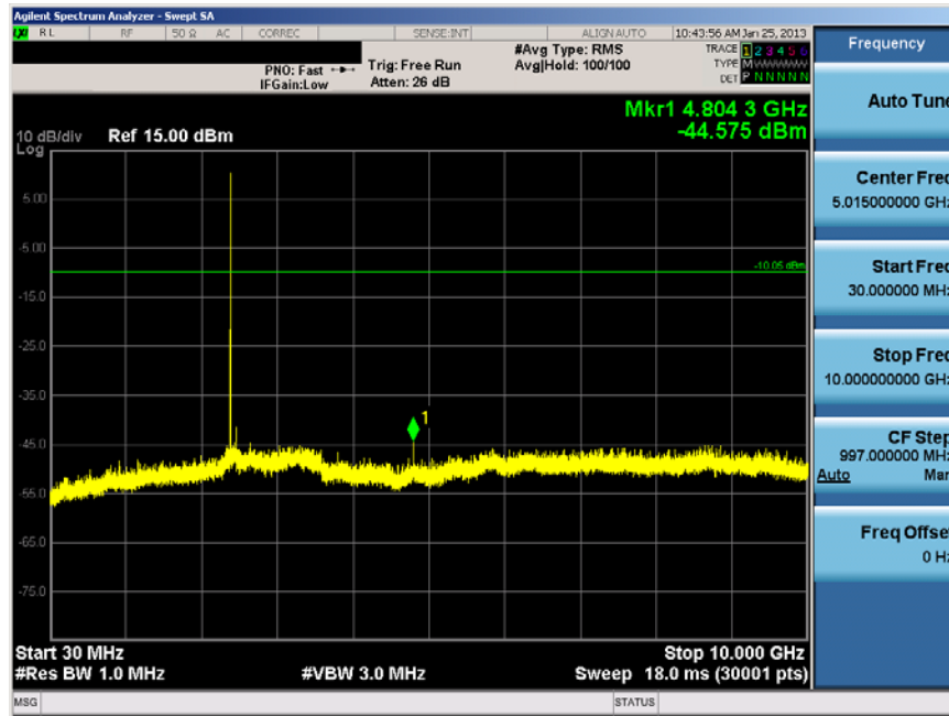
Plot 6-36. Conducted Spurious Plot (Bluetooth, 1Mbps – Ch. 0)
