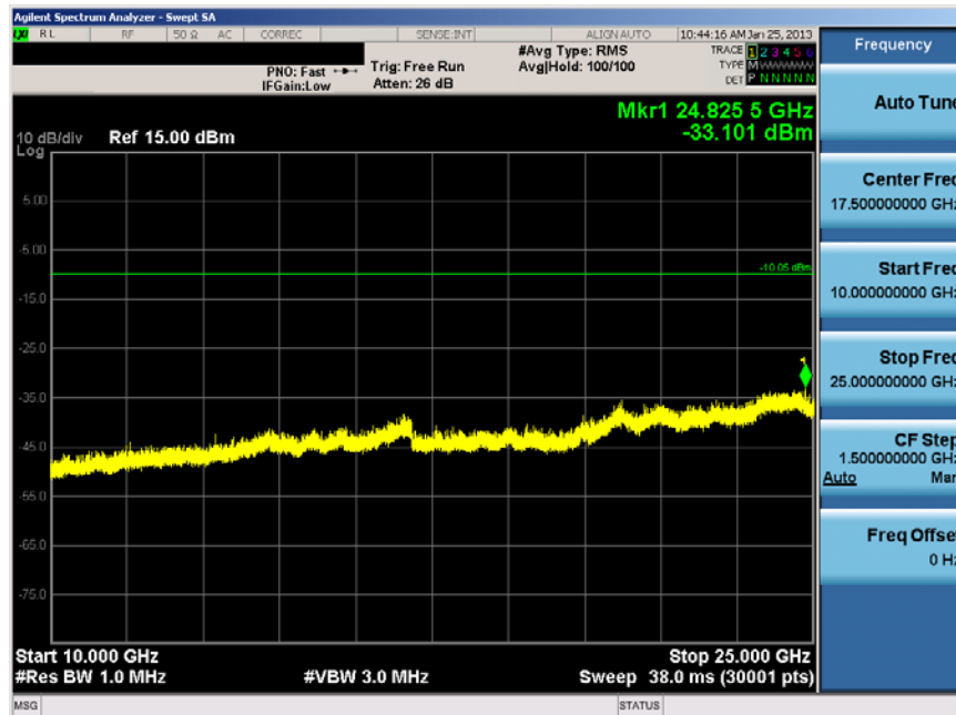
Plot 6-37. Conducted Spurious Plot (Bluetooth, 1Mbps – Ch. 0)
