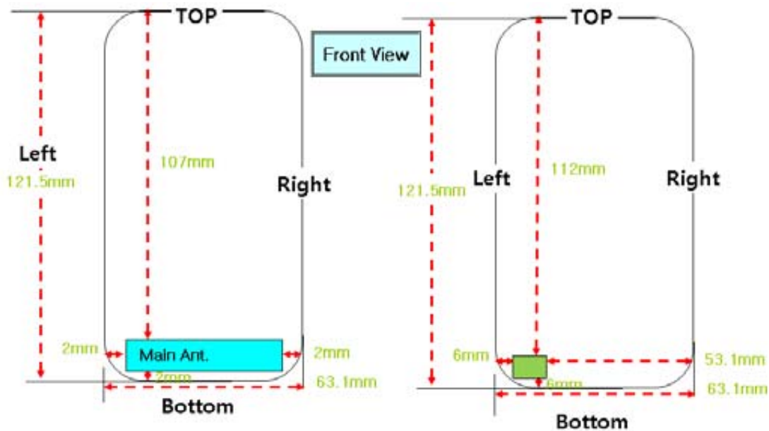
Figure 5.7 Identification of Sides for SAR Testing
