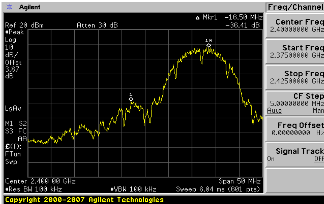
Plot 6-13. Band Edge Plot (802.11b – Ch. 1)
