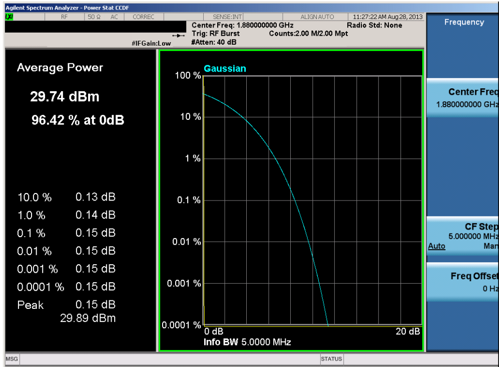
Plot 6-40. Peak-Average Ratio Plot (PCS GSM Mode – Ch. 661)
