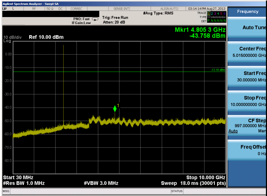
Plot 6-12. Conducted Spurious Plot (Bluetooth (LE) – Ch. 0)
