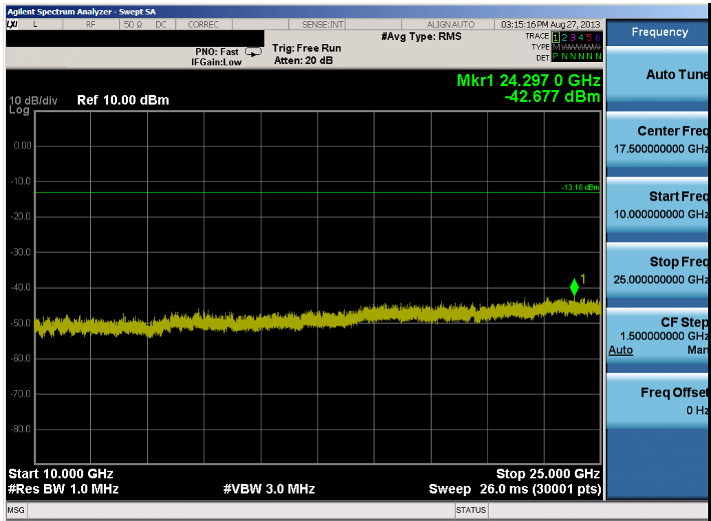
Plot 6-13. Conducted Spurious Plot (Bluetooth (LE) – Ch. 0)
