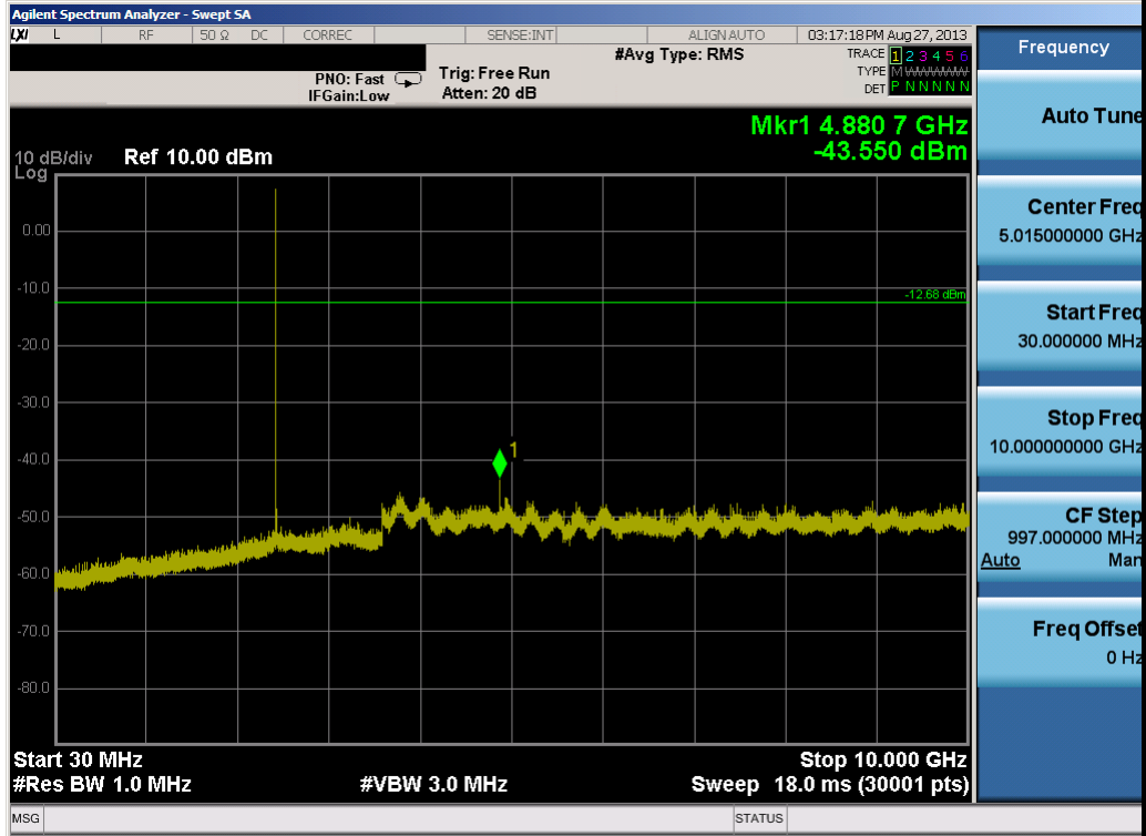
Plot 6-14. Conducted Spurious Plot (Bluetooth (LE) – Ch. 19)
