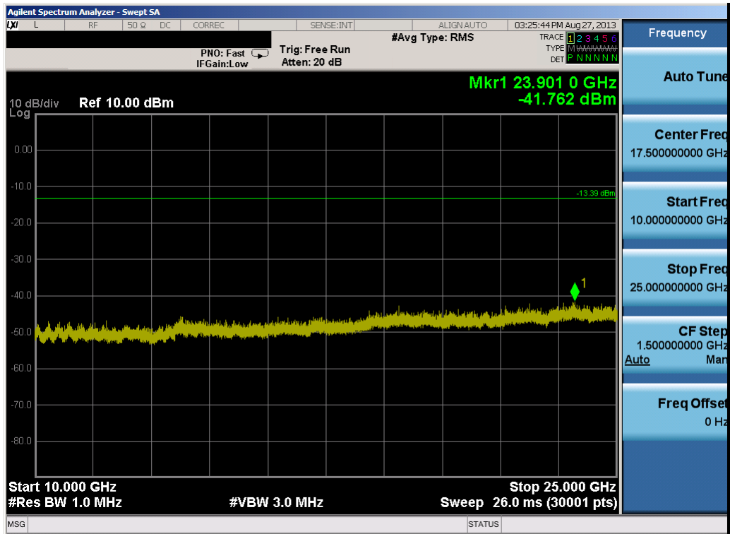
Plot 6-17. Conducted Spurious Plot (Bluetooth (LE) – Ch. 39)
