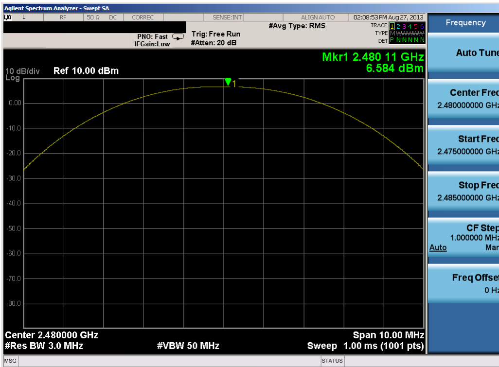
Plot 6-6. Peak Power Plot (Bluetooth (LE) – Ch. 39)
