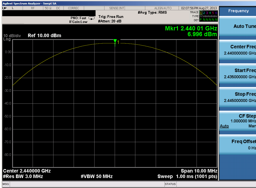
Plot 6-5. Peak Powery Plot (Bluetooth (LE) – Ch. 19)
