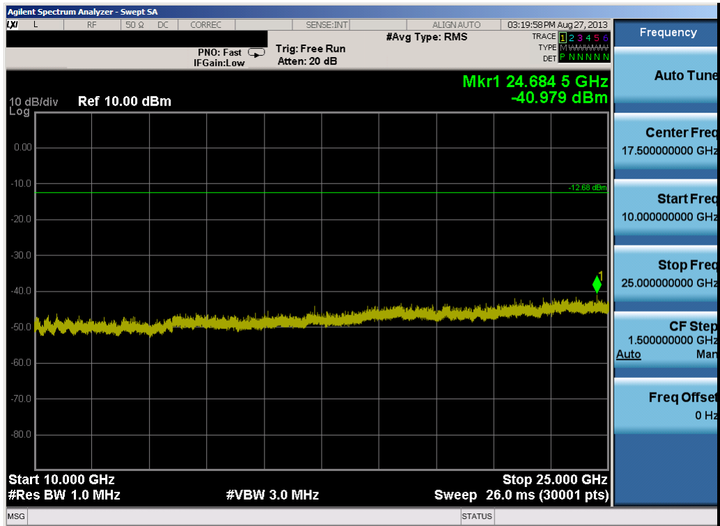
Plot 6-15. Conducted Spurious Plot (Bluetooth (LE) – Ch. 19)
