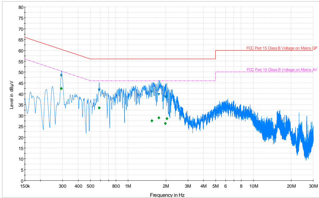
— FCC Part 15 Class B Voltage on Mains OP.LimitLine - - - FCC Part 15 Class B Voltage on Mains AV.LimitLine — Preview Result 1-PK+ ▲ Final Result 1-QPK ◆ Final Result 2-AVG
