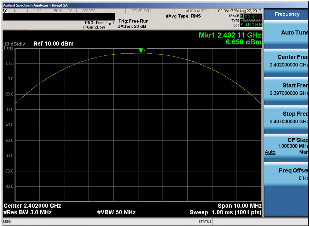
Plot 6-4. Peak Power Plot (Bluetooth (LE) – Ch. 0)
