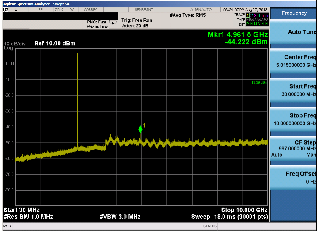
Plot 6-16. Conducted Spurious Plot (Bluetooth (LE) – Ch. 39)
