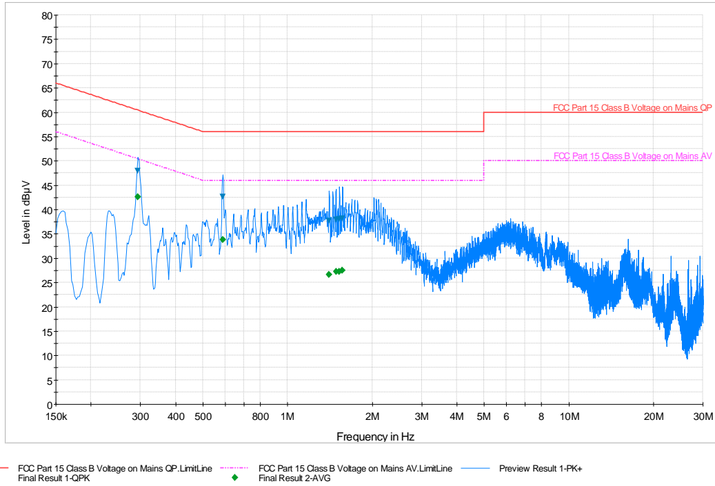
Plot 6-36. Line Conducted Plot with 802.11b (N)
