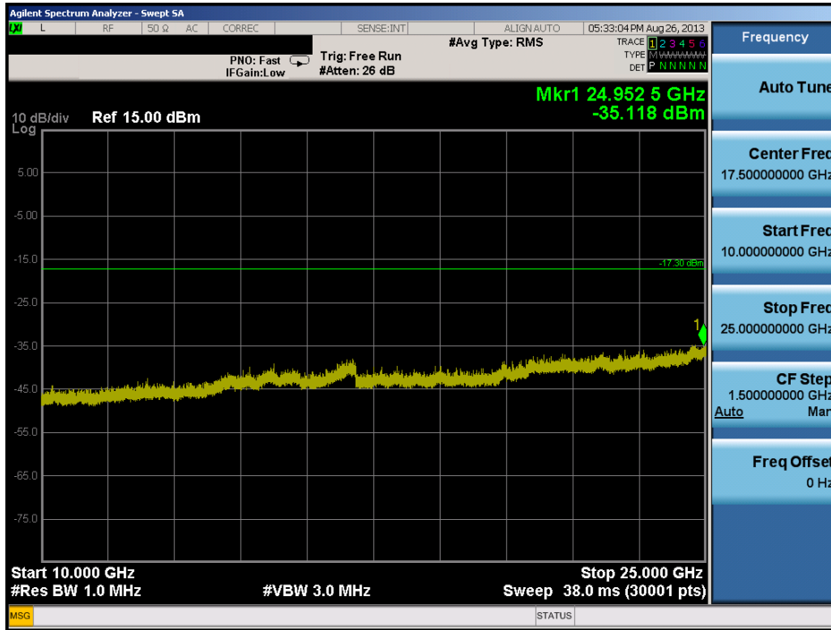
Plot 6-28. Conducted Spurious Plot (802.11b – Ch. 6)
