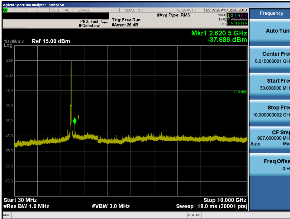
Plot 6-29. Conducted Spurious Plot (802.11b – Ch. 11)
