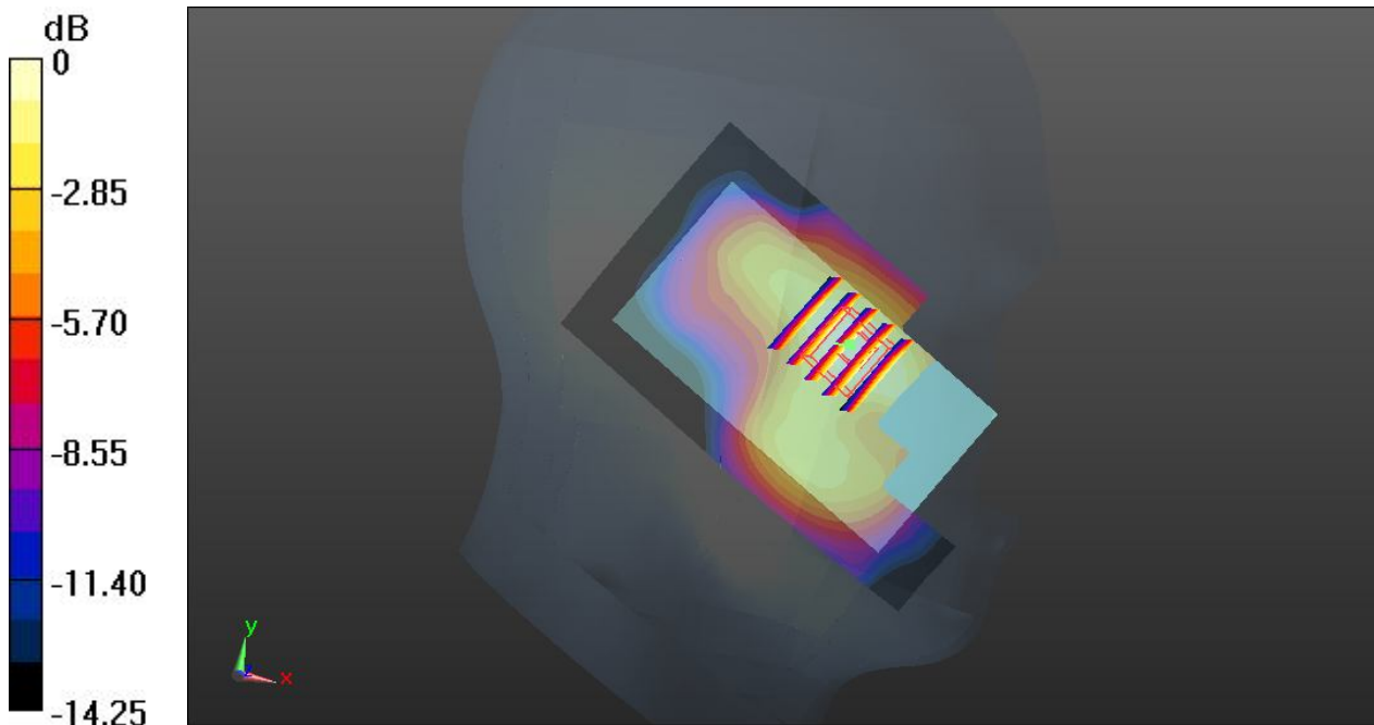
0 dB = 0.311 W/kg
