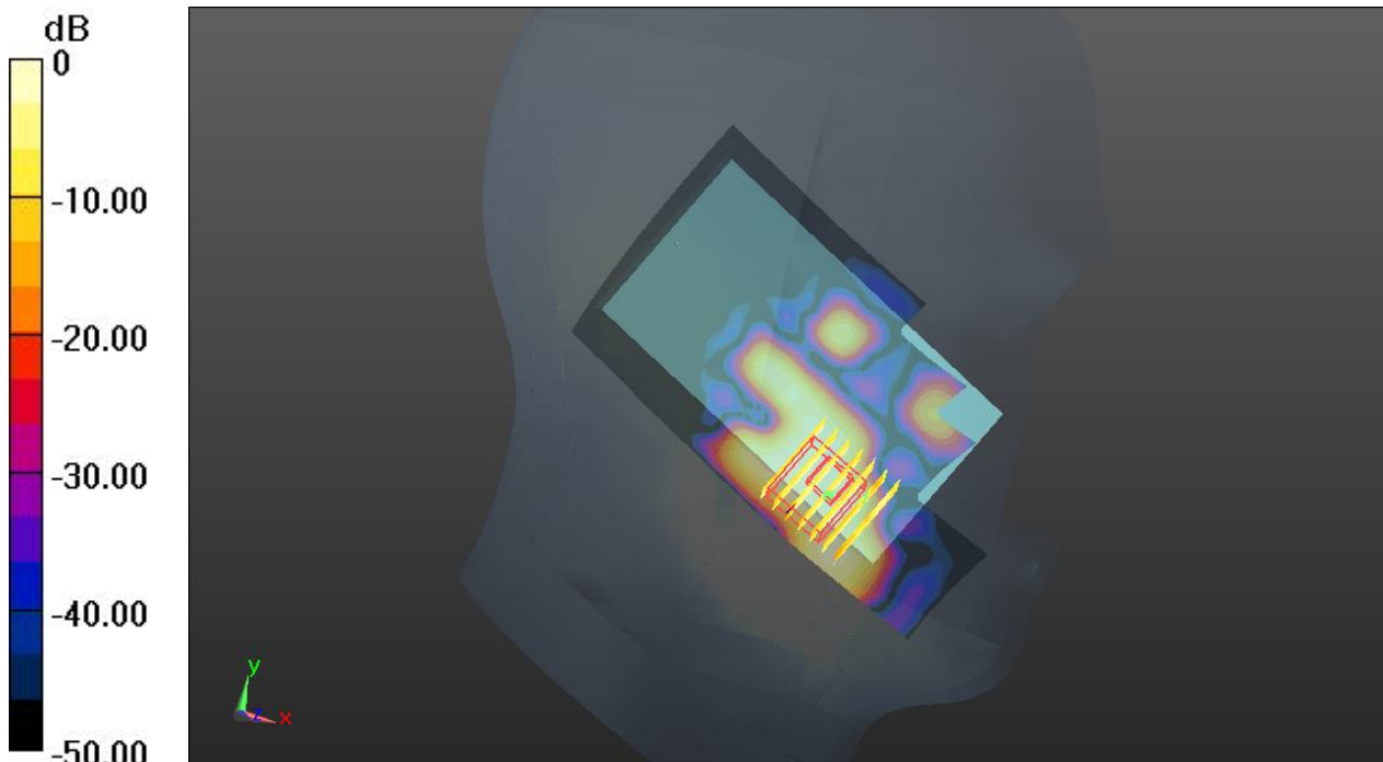
0 dB = 0.0457 W/kg
