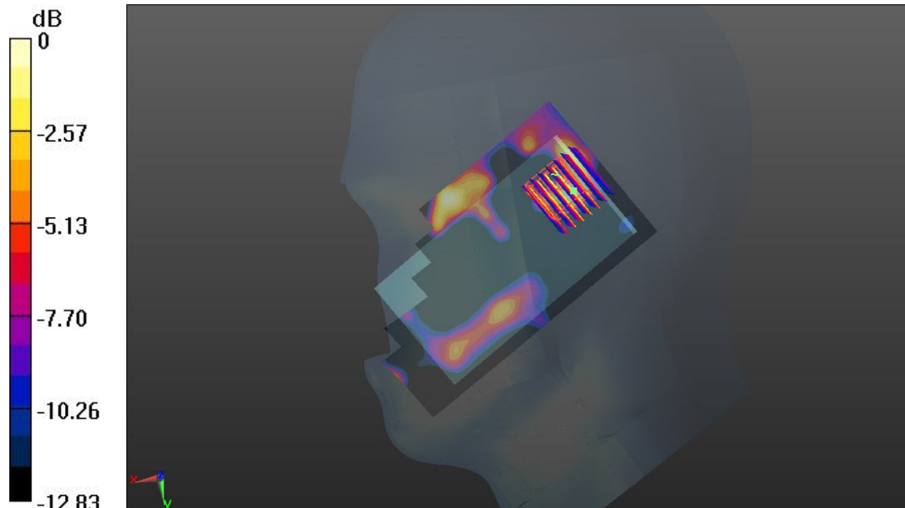
0 dB = 0.0402 W/kg
