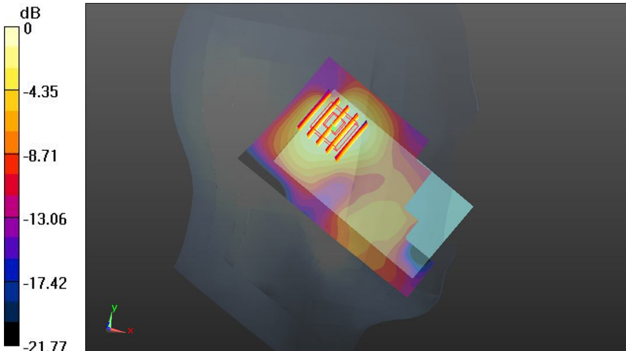
0 dB = 0.180 W/kg
