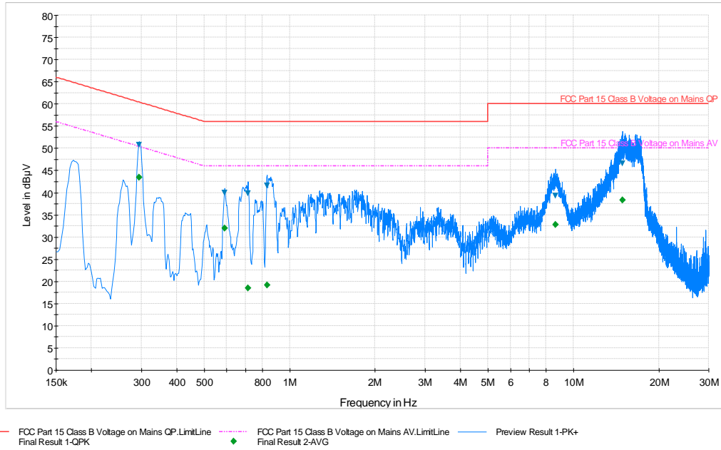
Plot 6-35. Line Conducted Plot with 802.11b (L1)
