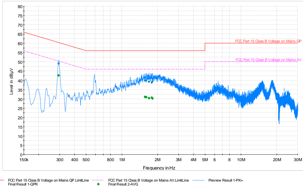
Plot 6-36. Line Conducted Plot with 802.11b (N)
