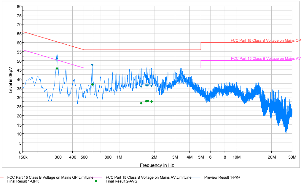
Plot 6-36. Line Conducted Plot with 802.11b (N)
