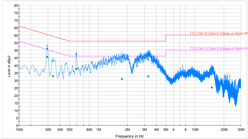
— FCC Part 15 Class B Voltage on Mains QP.LimitLine — FCC Part 15 Class B Voltage on Mains AV.LimitLine — Preview Result 1-QP+ Final Result 1-QPK ▲ Final Result 1-QPK ◆ Final Result 2-AVG
