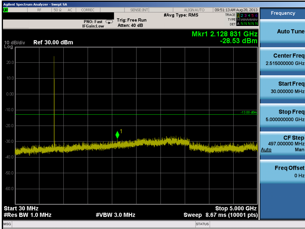
Plot 8-6. Conducted Spurious Plot (10.0MHz QPSK – RB Size 1, RB Offset 0 – Mid Channel)
