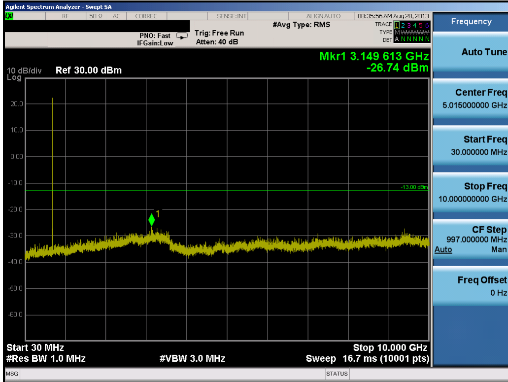
Plot 7-16. Conducted Spurious Plot (5.0MHz QPSK – RB Size 1, RB Offset 0 – Mid Channel)
