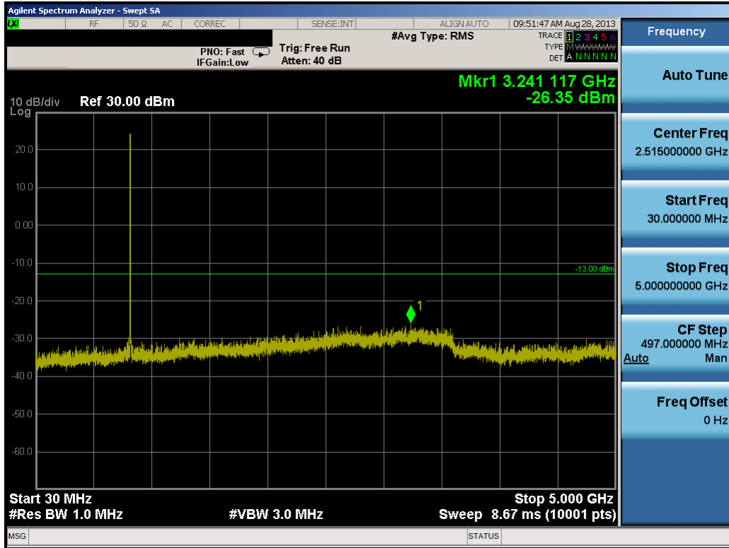
Plot 8-8. Conducted Spurious Plot (10.0MHz QPSK – RB Size 1, RB Offset 0 – High Channel)
