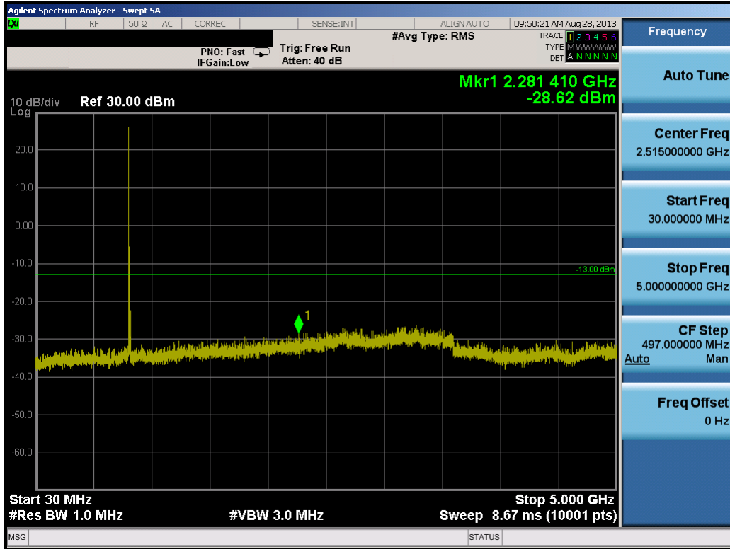
Plot 8-4. Conducted Spurious Plot (10.0MHz QPSK – RB Size 1, RB Offset 0 – Low Channel)
