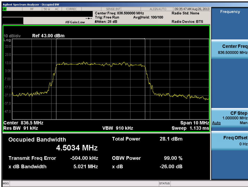
Plot 8-17. Occupied Bandwidth Plot (5.0MHz 16-QAM – RB Size 25)
