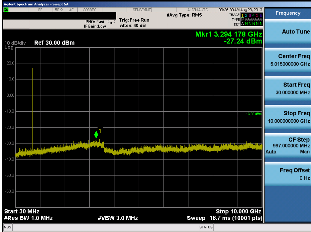
Plot 7-14. Conducted Spurious Plot (5.0MHz QPSK – RB Size 1, RB Offset 0– Low Channel)
