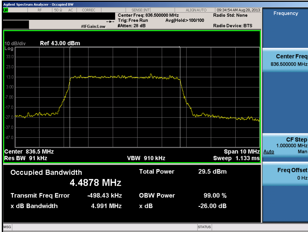
Plot 8-16. Occupied Bandwidth Plot (5.0MHz QPSK – RB Size 25)
