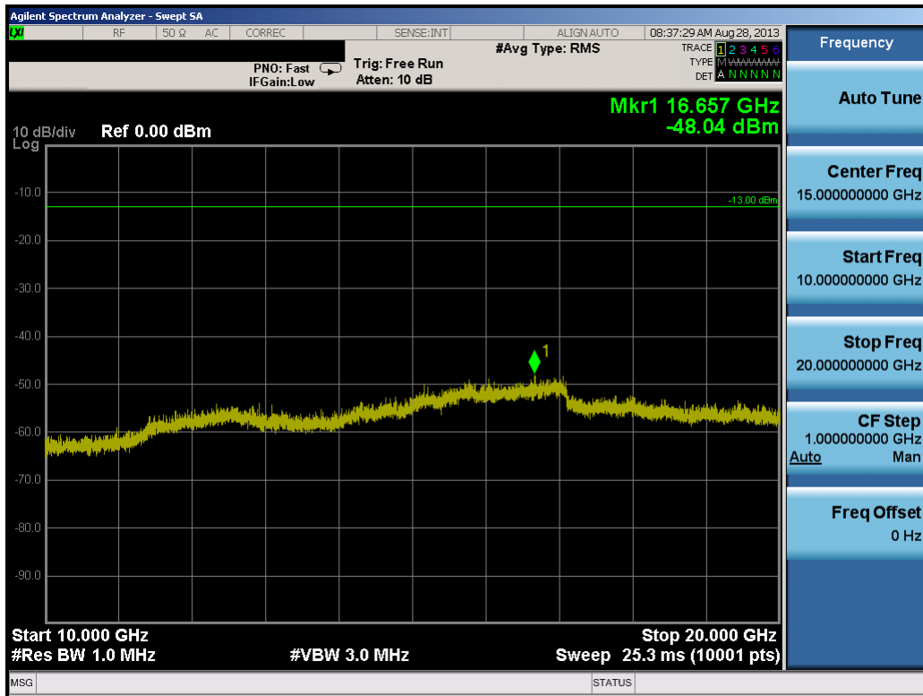
Plot 7-17. Conducted Spurious Plot (5.0MHz QPSK – RB Size 1, RB Offset 0 – Mid Channel)
