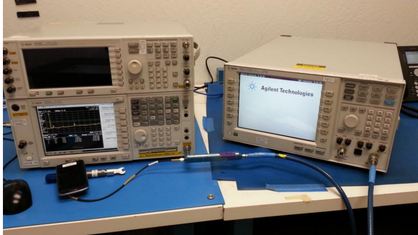
ANTENNA PORT CONDUCTED PHOTO
