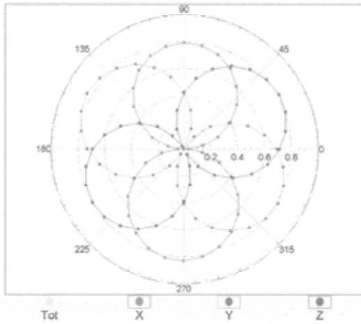
f=600 MHz,TEM
