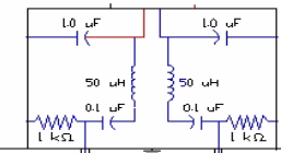
Figure 3-4. LISN Schematic Diagram
