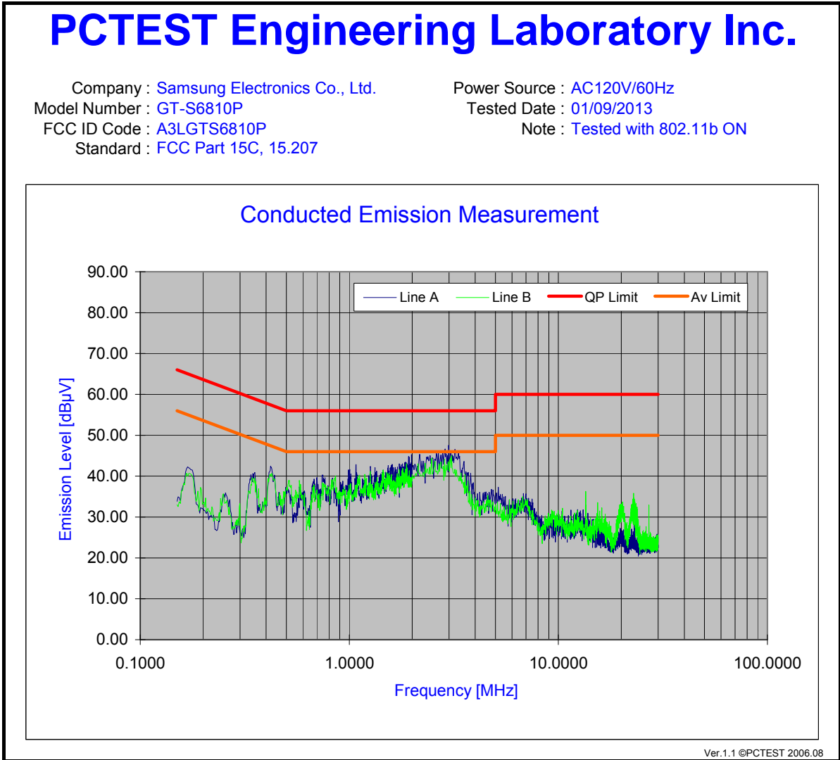
Plot 6-33. Line Conducted Plot with 802.11b
