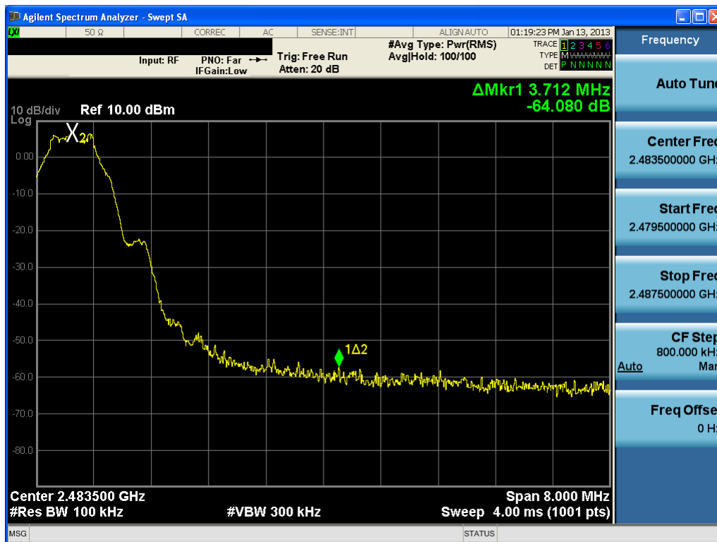
Plot 6-9. Band Edge Plot (Bluetooth (LE) – Ch. 39)
