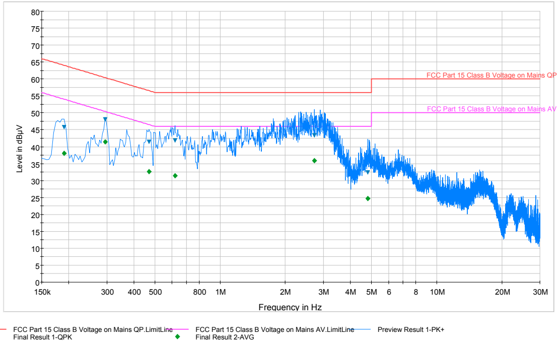
Plot 6-16. Line Conducted Plot with Bluetooth LE (L1)
