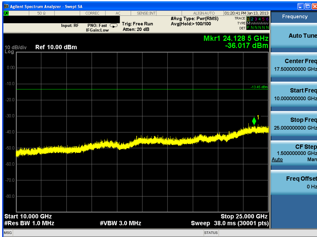
Plot 6-15. Conducted Spurious Plot (Bluetooth (LE) – Ch. 39)
