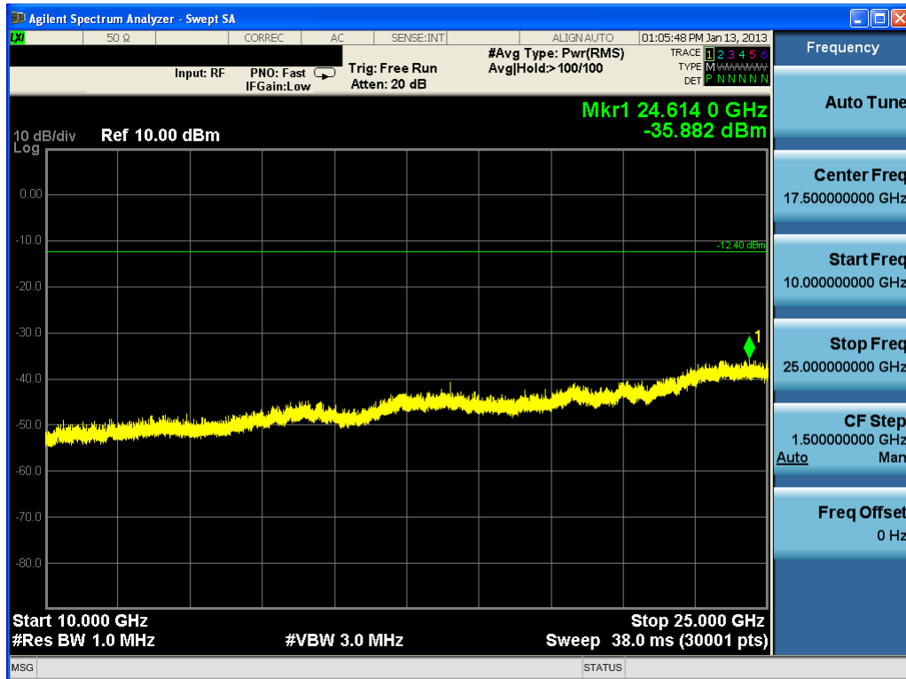
Plot 6-11. Conducted Spurious Plot (Bluetooth (LE) – Ch. 0)
