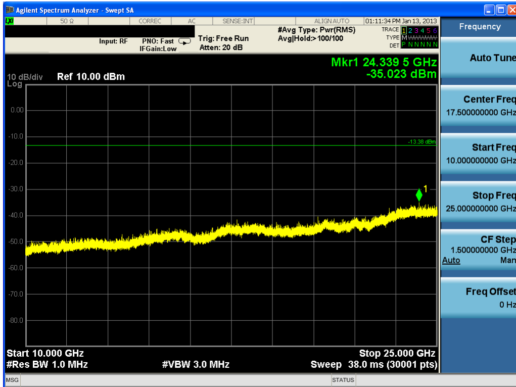
Plot 6-13. Conducted Spurious Plot (Bluetooth (LE) – Ch. 19)
