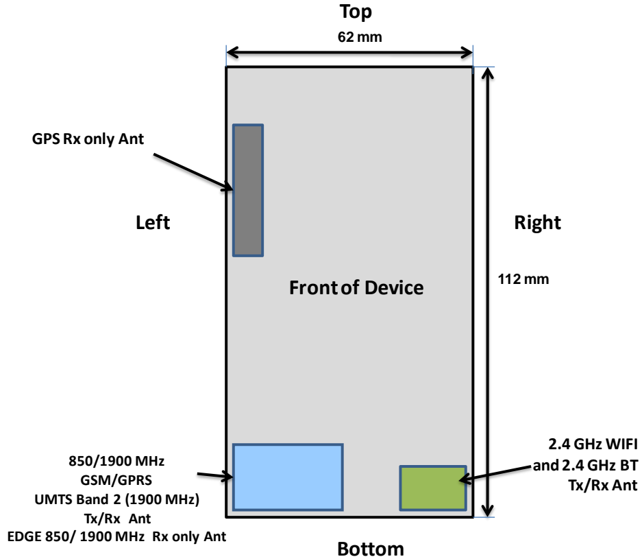
Figure 1-1 DUT Antenna Locations
