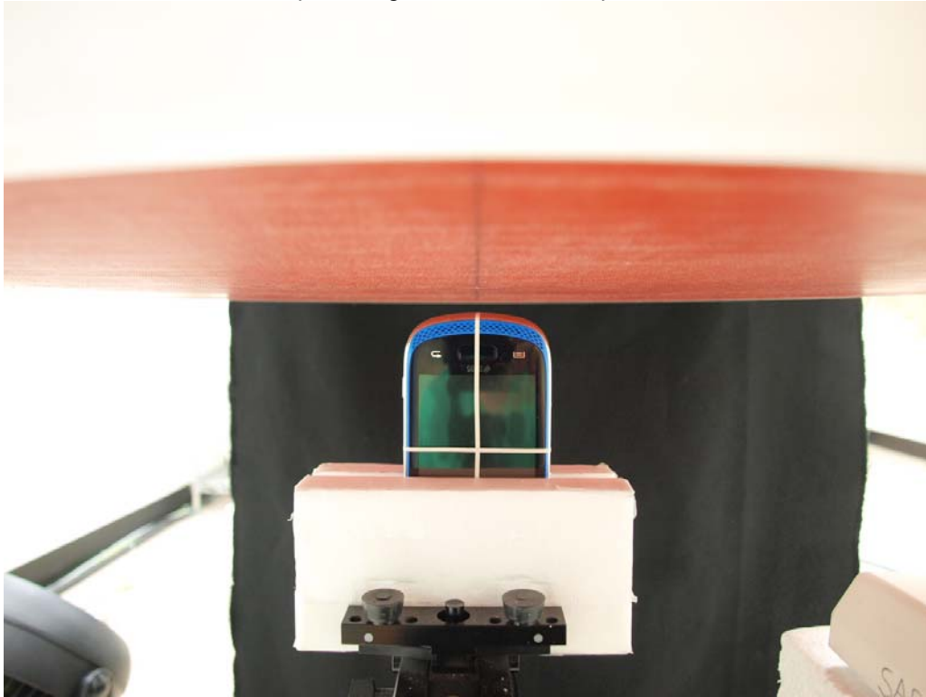
Hotspot - Edge 4 with 10 mm Separation
