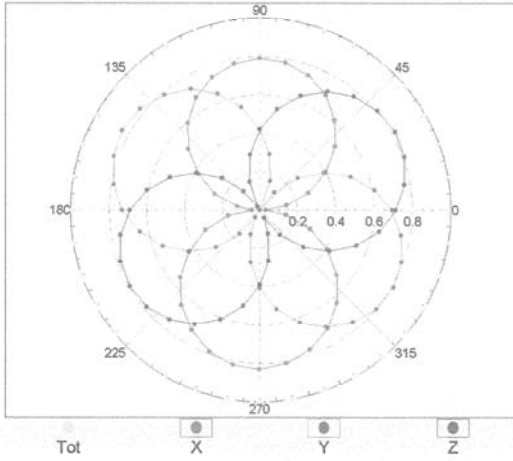
f=600 MHz,TEM
