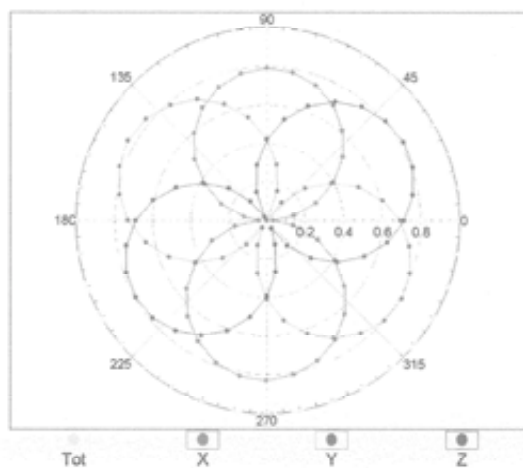
f=600 MHz,TEM
