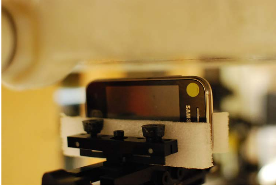
SAR Test Setup Photo 7 – Left at 1.0 cm
