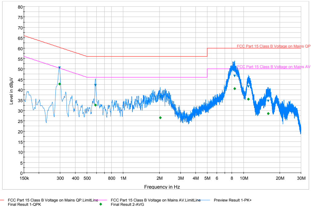
Plot 6-35. Line Conducted Plot with 802.11b (L1)
