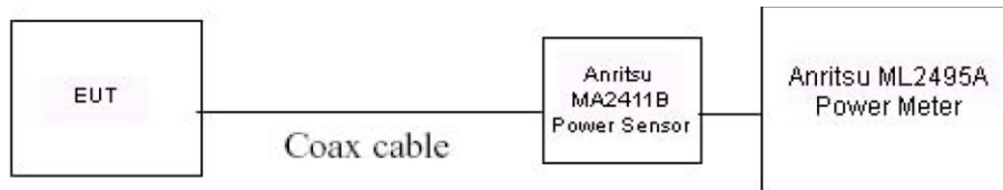
Figure 8-3 Power Measurement Setup
