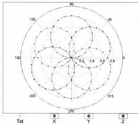
f=600 MHz,TEM
