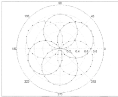
f=600 MHz,TEM
