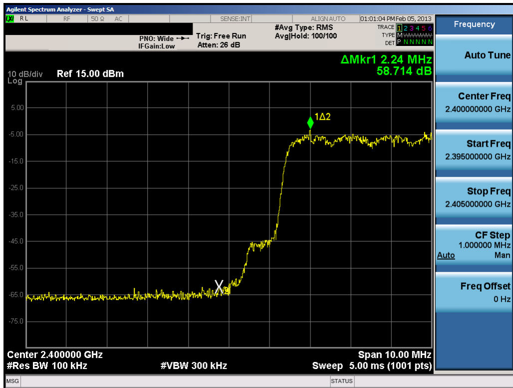
Plot 6-30. Band Edge Plot (Bluetooth with Hopping Enabled, 2Mbps)
