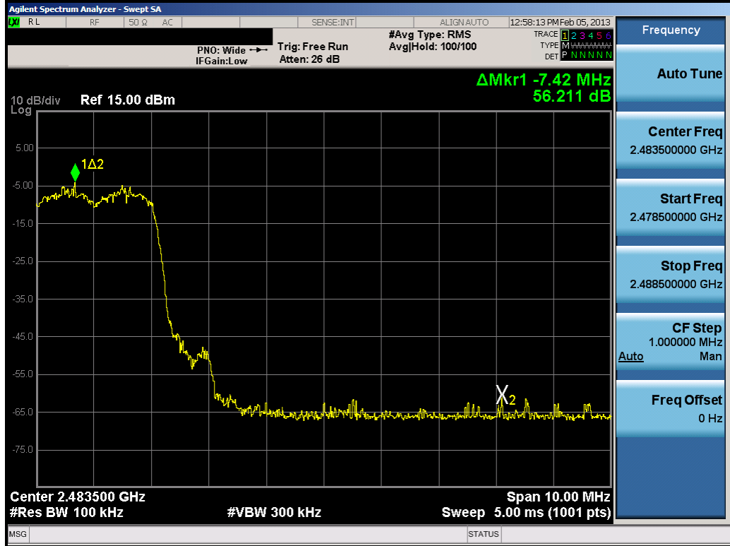
Plot 6-31. Band Edge Plot (Bluetooth with Hopping Enabled, 2Mbps)
