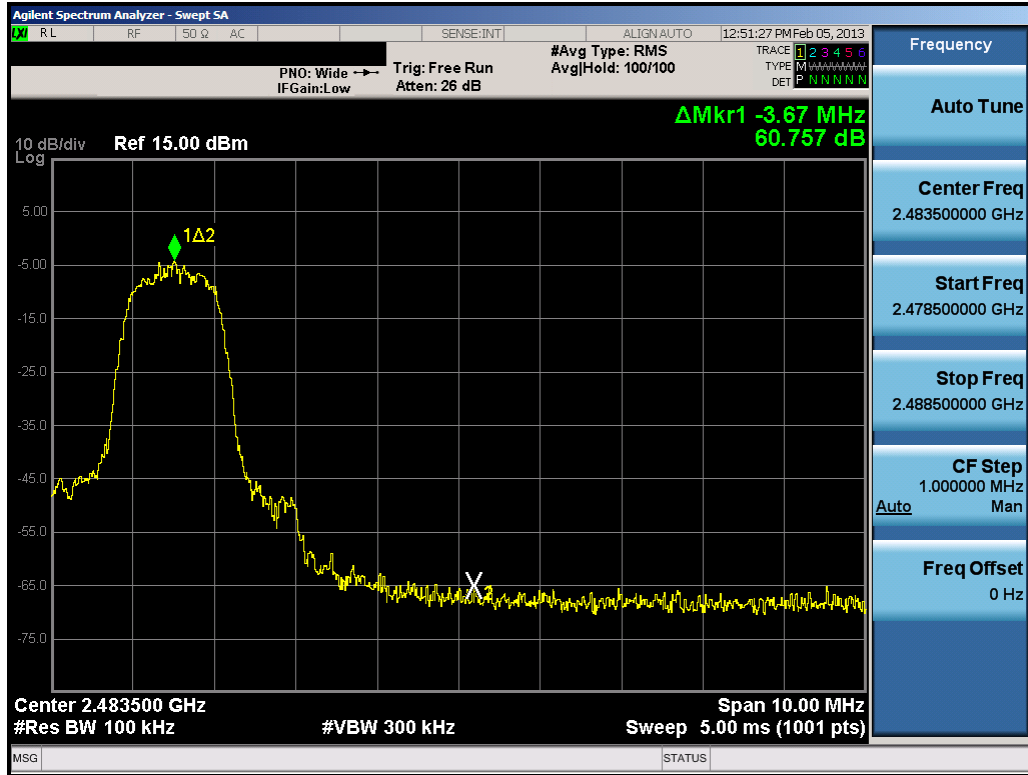
Plot 6-29. Band Edge Plot (Bluetooth with Hopping Disabled, 2Mbps – Ch. 78)
