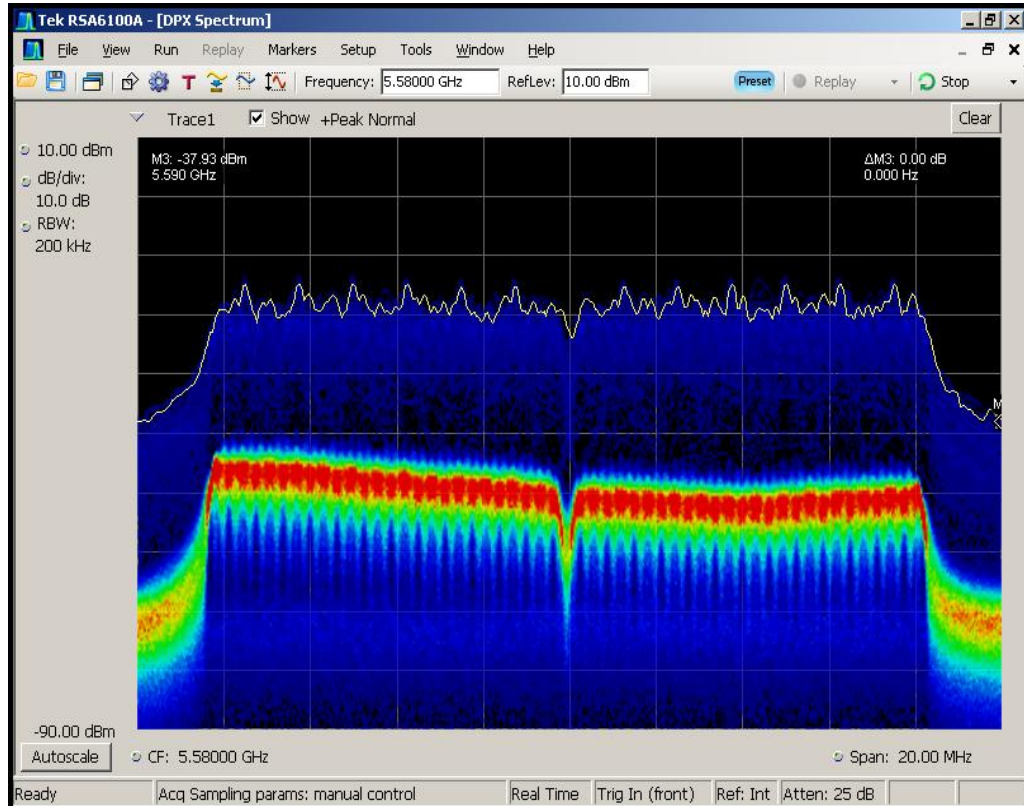
Figure 6-4. Real-Time Spectrum Display, WLAN Traffic (Streaming Video)
