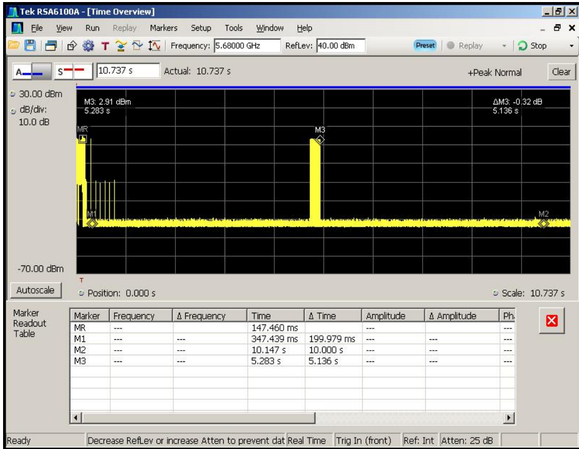
Figure 6-5. Channel Move Time (< 10sec)
