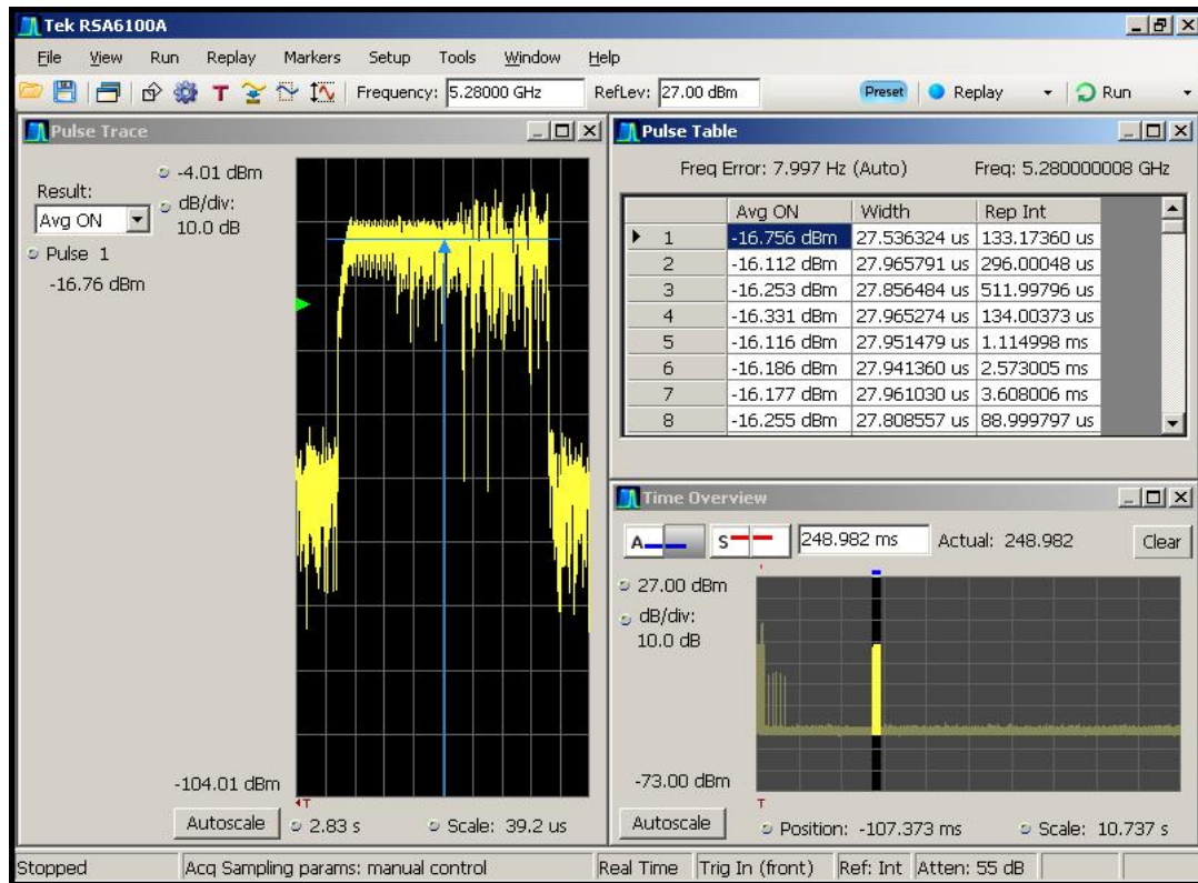
Figure 5-6. Aggregate Time using Pulse Table Capability
