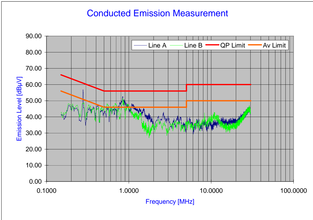
Plot 6-55. Line Conducted Plot with 802.11g
