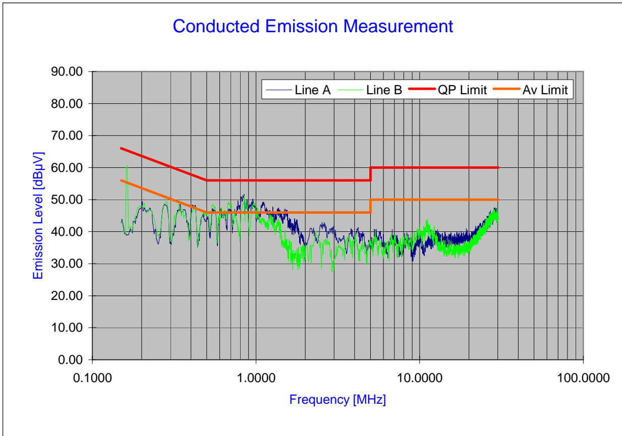
Plot 6-54. Line Conducted Plot with 802.11b
