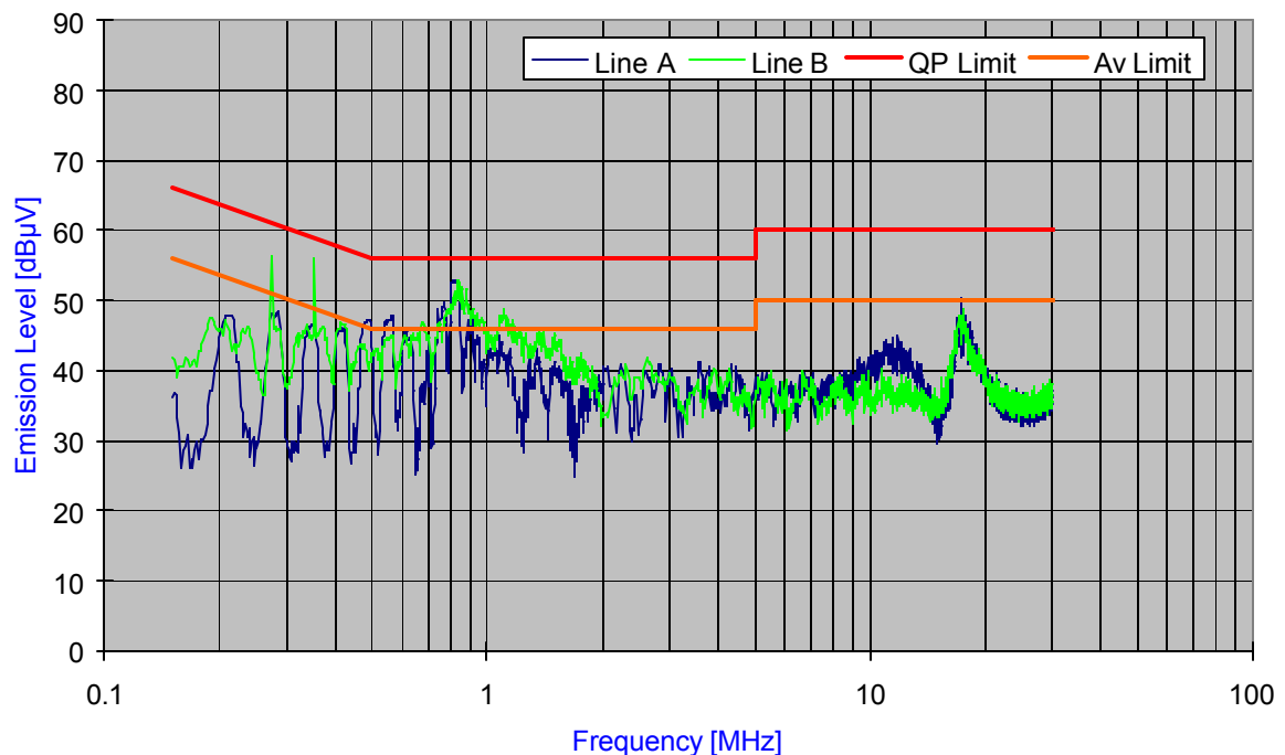
Plot 6-57. Line Conducted Plot with 802.11a (UNII Band 3)
