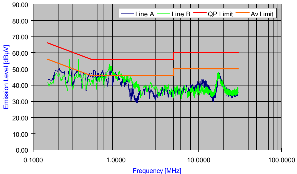
Plot 6-55. Line Conducted Plot with 802.11a (UNII Band 1)
