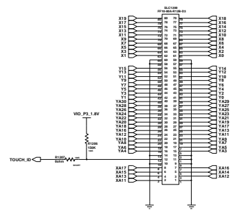
<80Pin TOUCH Con.>
