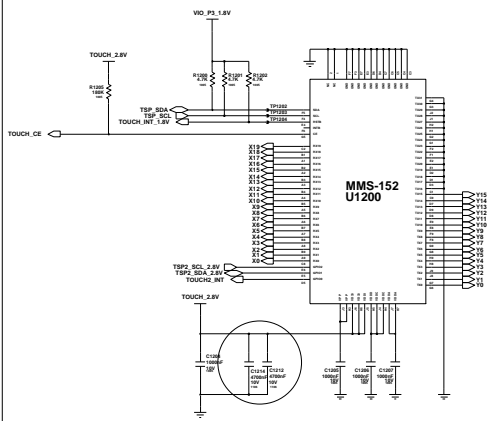
<TOCH SENSOR IC>
