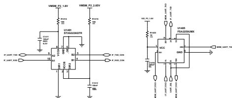
<UART SWITCH>
