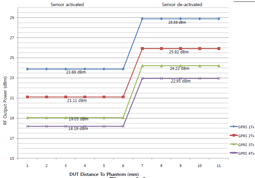
Figure 9-9 GPRS 1900 Back off Power Reduction Graph - Top Edge at 60° Angle
