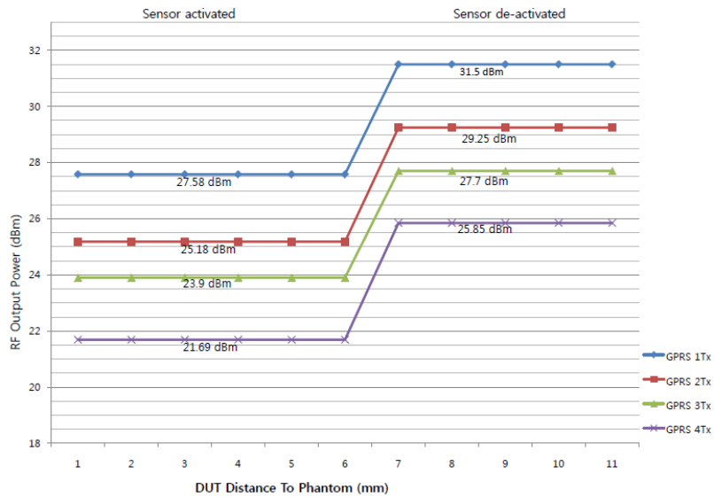
Figure 9-12 GPRS 850 Back off Power Reduction Graph - Left Edge at 60° Angle
