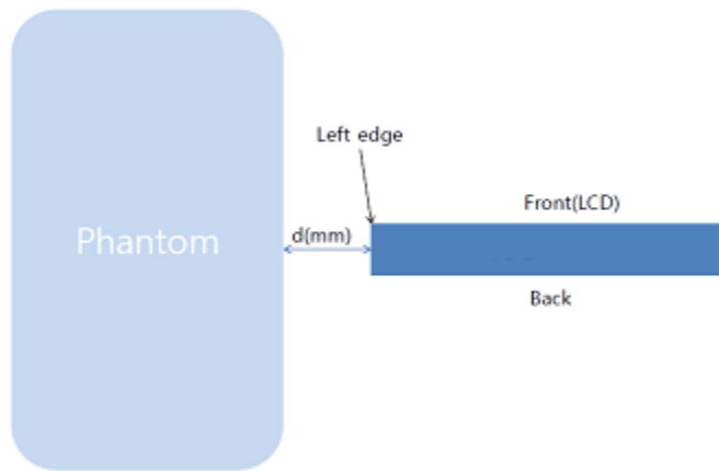
Backoff Sensor Power Reduction (Left side, 0° tilted)
