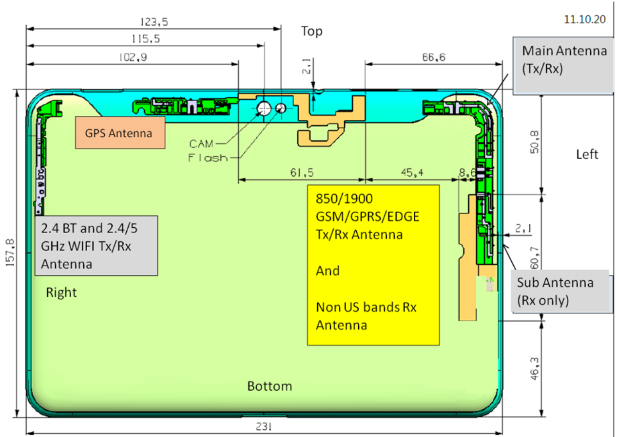
Figure 9-2 Back View of Device
