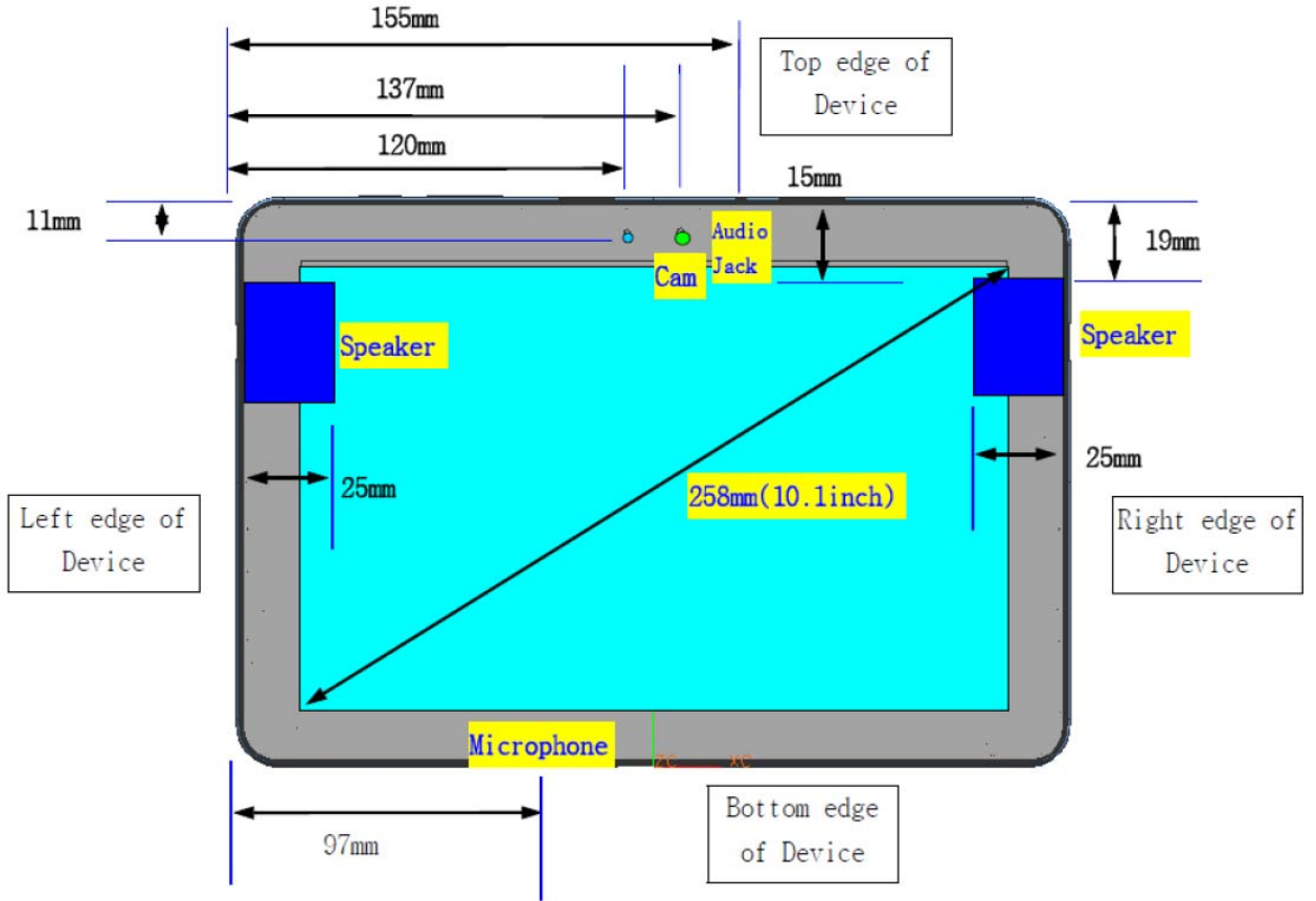
Figure 1-1. Front view of device
