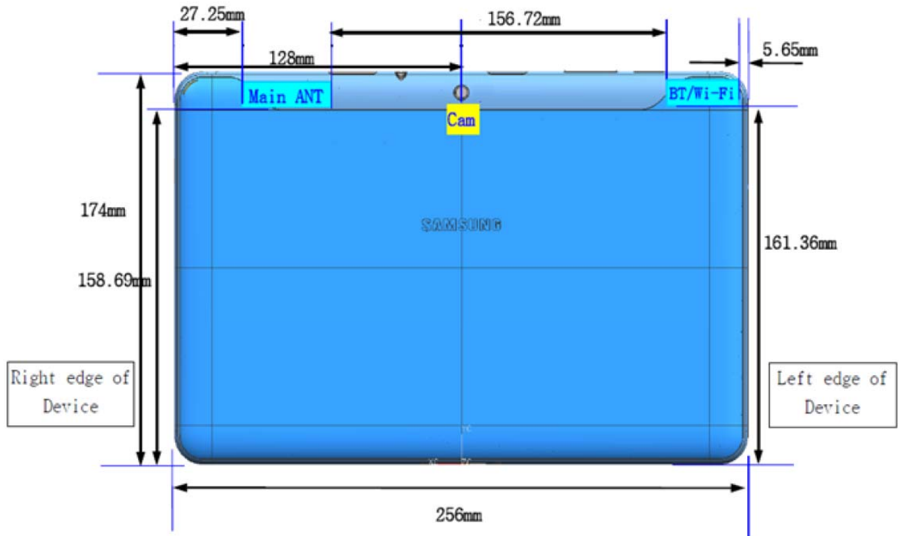
Figure 2. Back view of device
