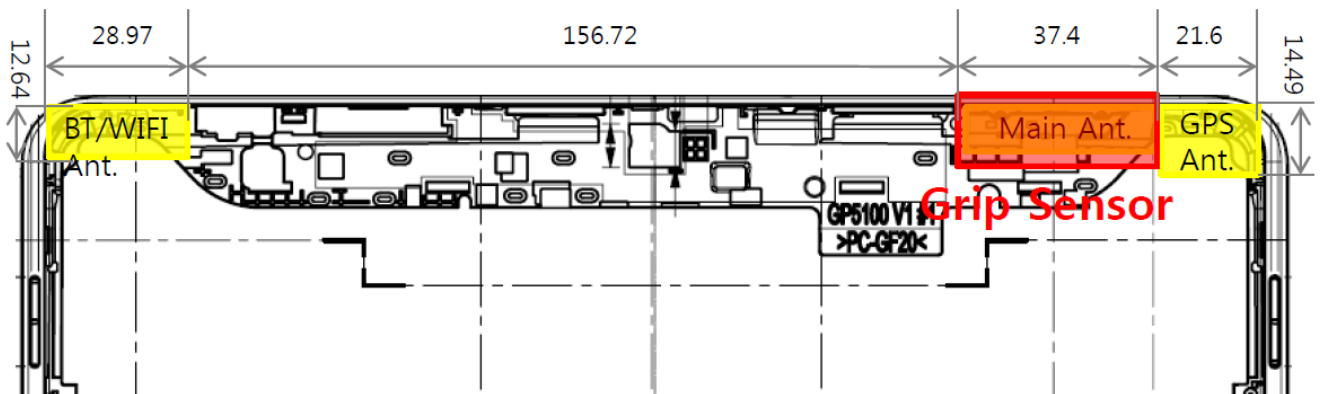
Figure 1-1. Front view of device
