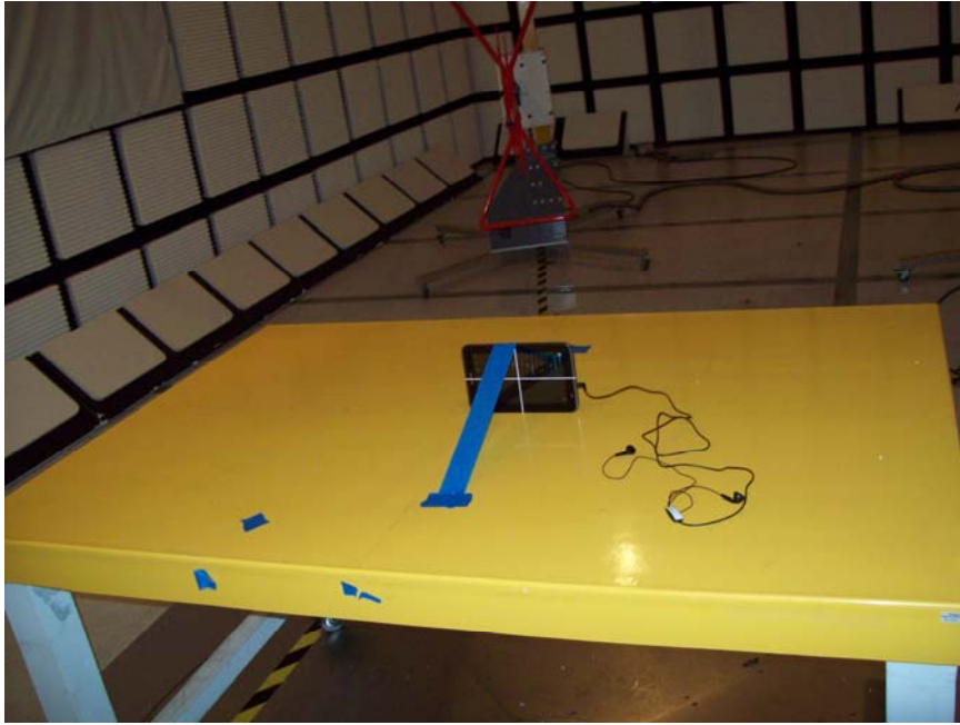
Y-AXIS WITH HEADSET FRONT PHOTO
