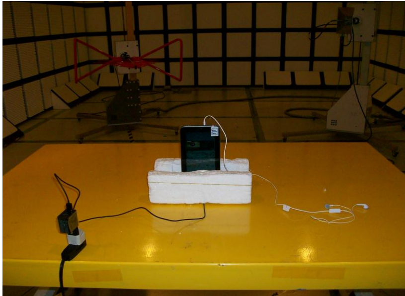
Y-AXIS PHOTO
