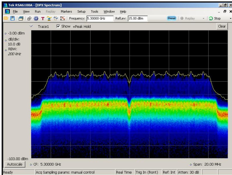
Figure 5-2. Real-Time Spectrum Display, WLAN Traffic (Streaming Video)
