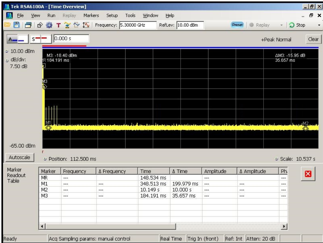
Figure 5-3. Channel Move Time (< 10sec)
