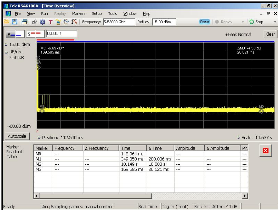
Figure 6-3. Channel Move Time (< 10sec)
