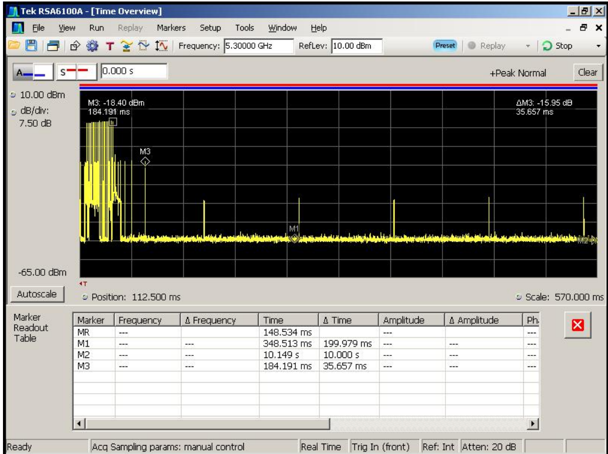
Figure 5-4. Zoomed-in Plot near M3
