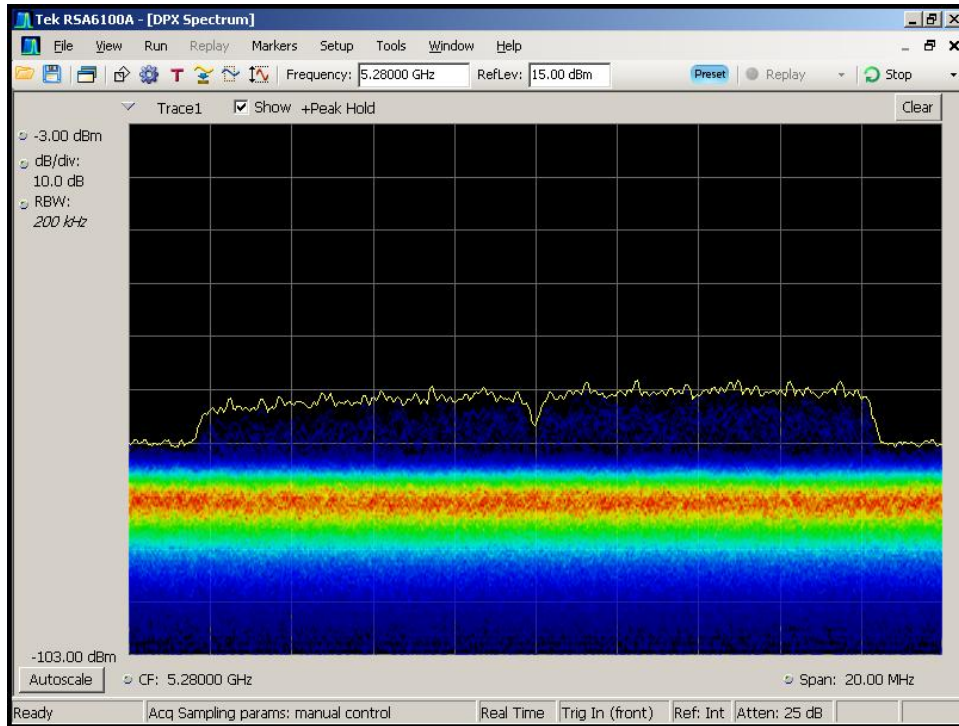
Figure 5-1. Real-Time Spectrum Display, No WLAN Traffic
