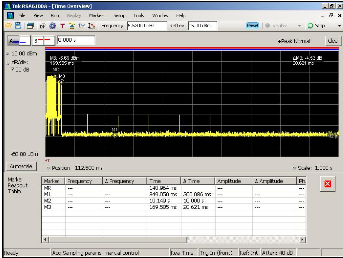
Figure 6-4. Zoomed-in Plot near M3
