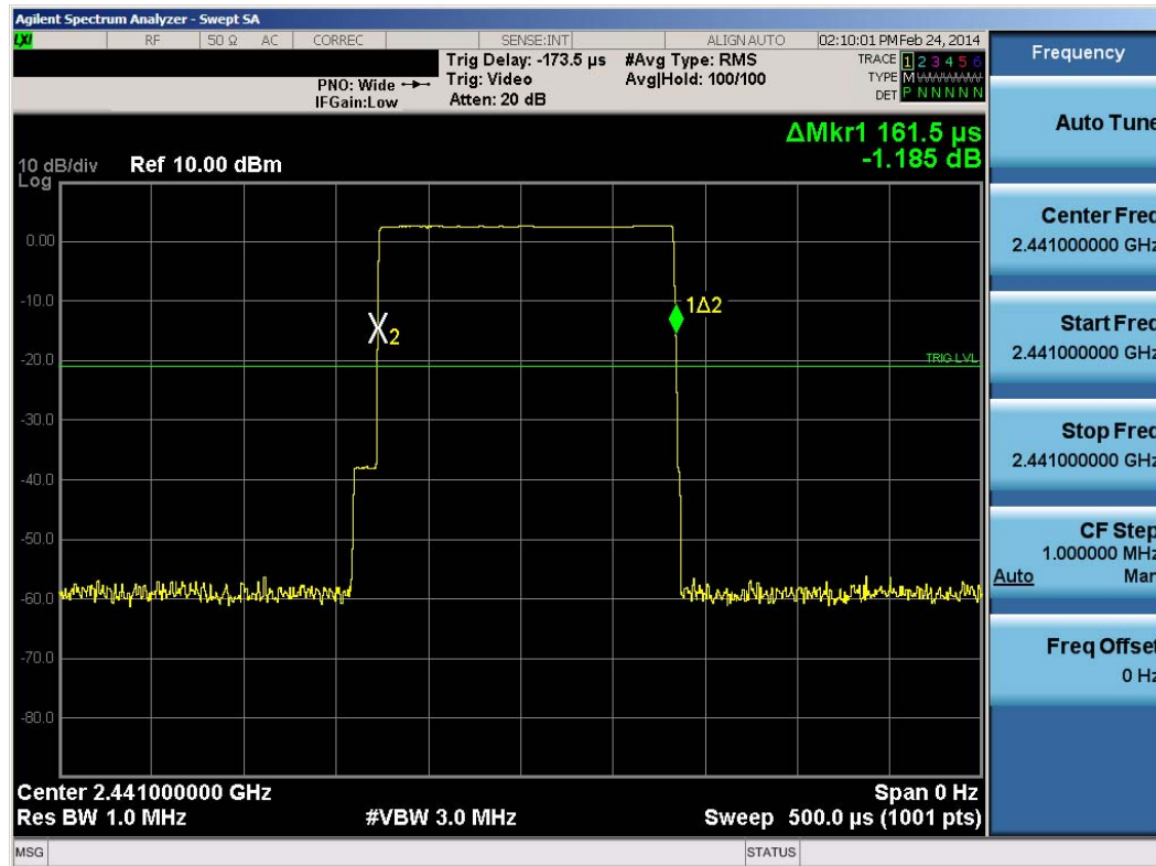
Plot 6-2. Pulse Width Measurement
