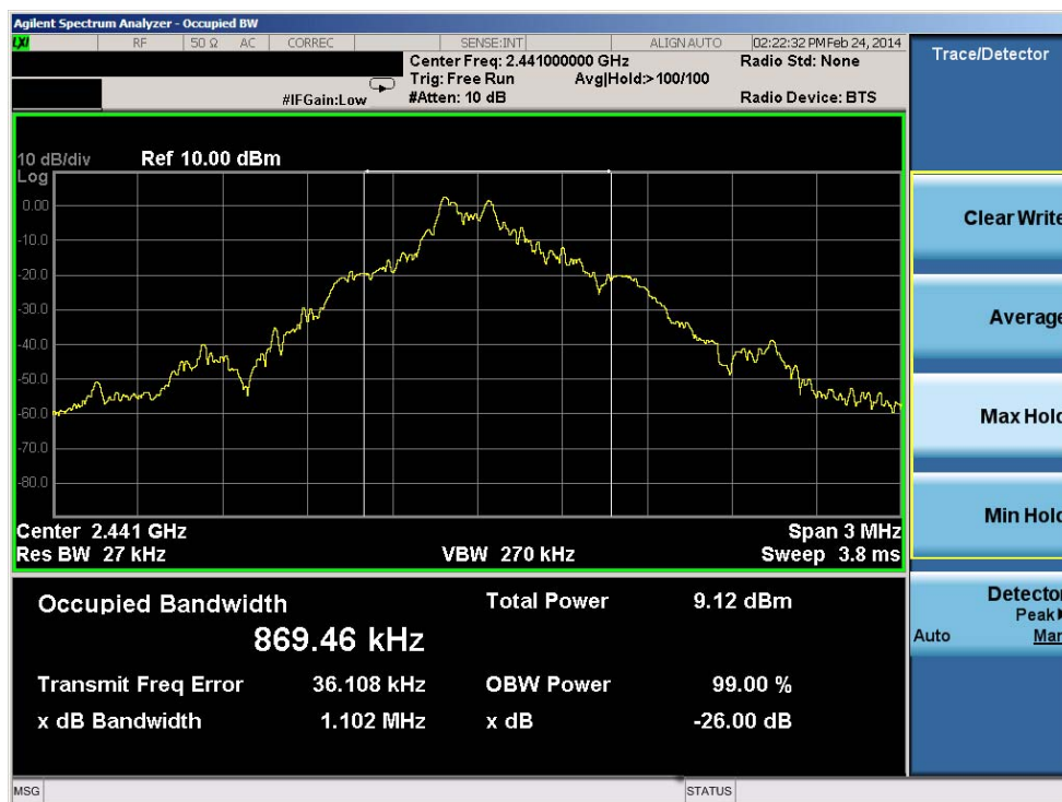
Plot 6-1. Occupied Bandwidth Plot (ANT+ – Ch. 39)
