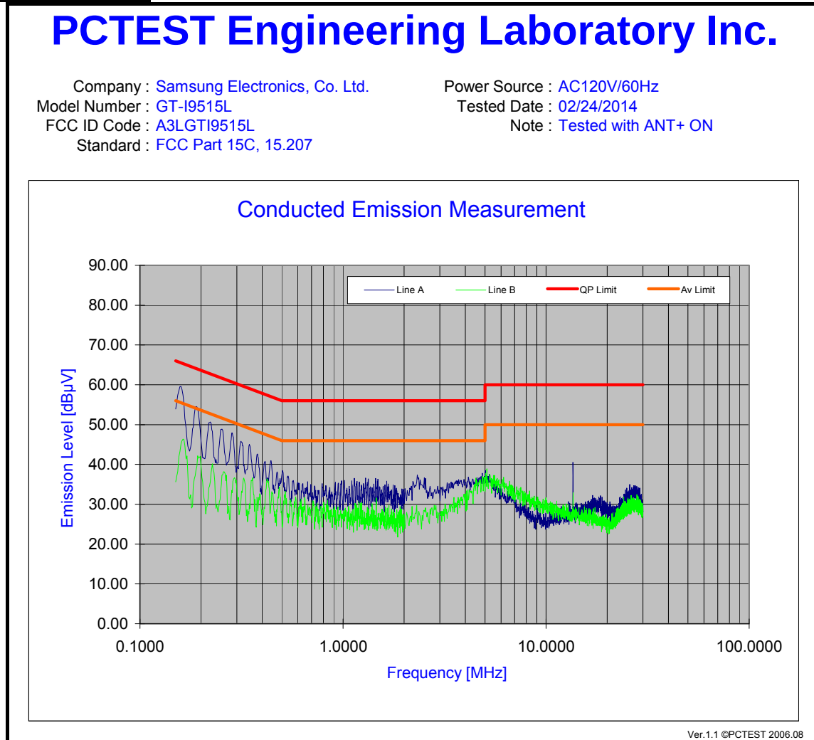
Plot 6-6. Line-Conducted Test Plot
