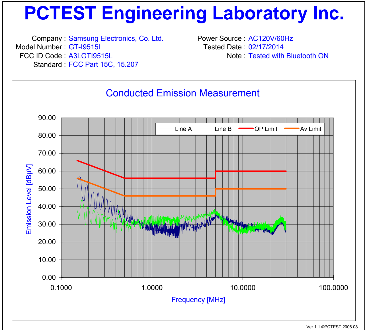
Plot 6-42. Line Conducted Plot with Bluetooth
