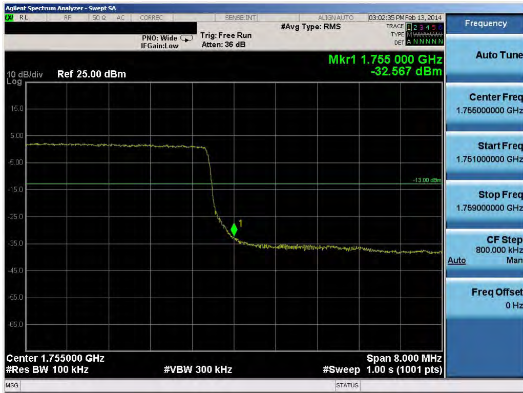
Plot 9-53. Upper Band Edge Plot (10.0MHz QPSK – RB Size 50)
