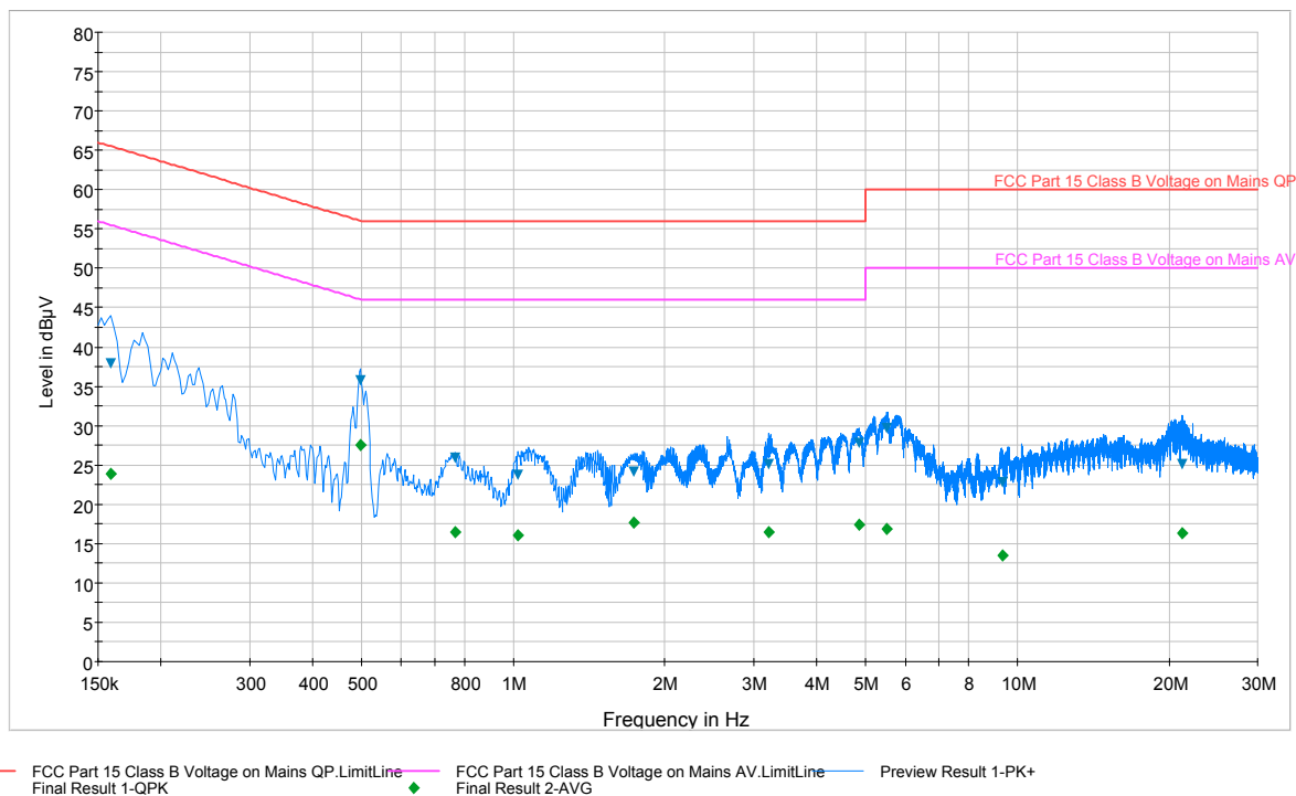
Plot 6-20. Line Conducted Plot with Bluetooth LE (L1)
