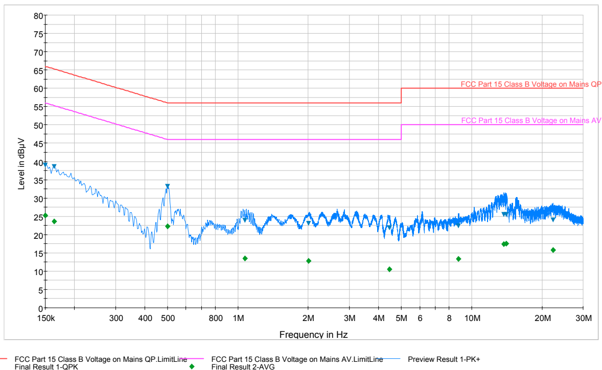
Plot 6-21. Line Conducted Plot with Bluetooth LE (N)
