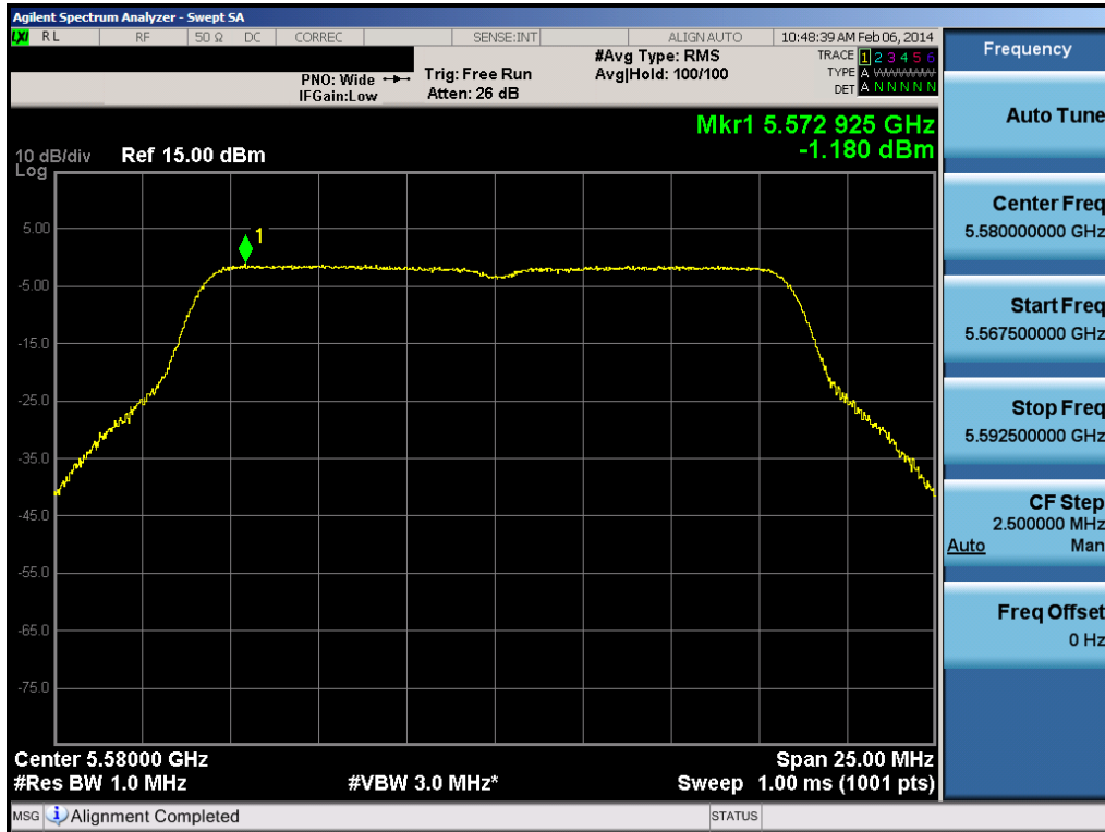
Plot 6-52. Peak Power Spectral Density Plot (802.11a (UNII Band 2C) – Ch. 116)
