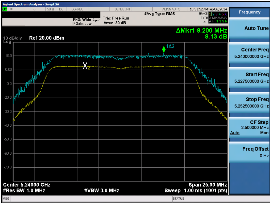
Plot 6-61. Peak Excursion Ratio Plot (802.11a)
