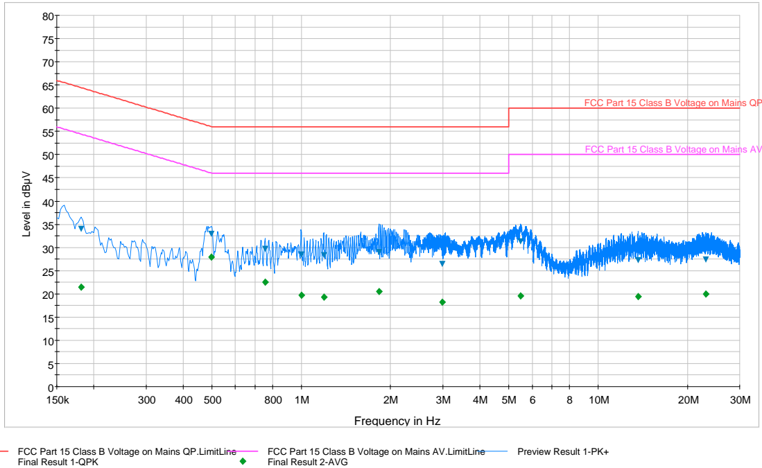
Plot 6-89. Line Conducted Plot with 802.11a UNII Band 2C (L1)
