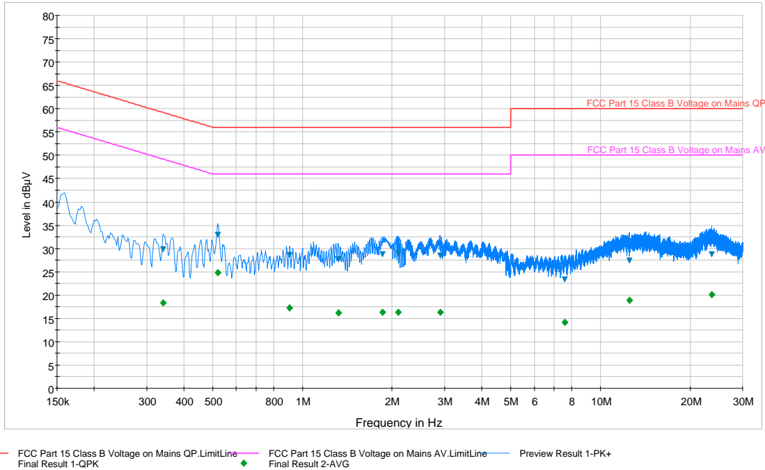
Plot 6-88. Line Conducted Plot with 802.11a UNII Band 2A (N)
