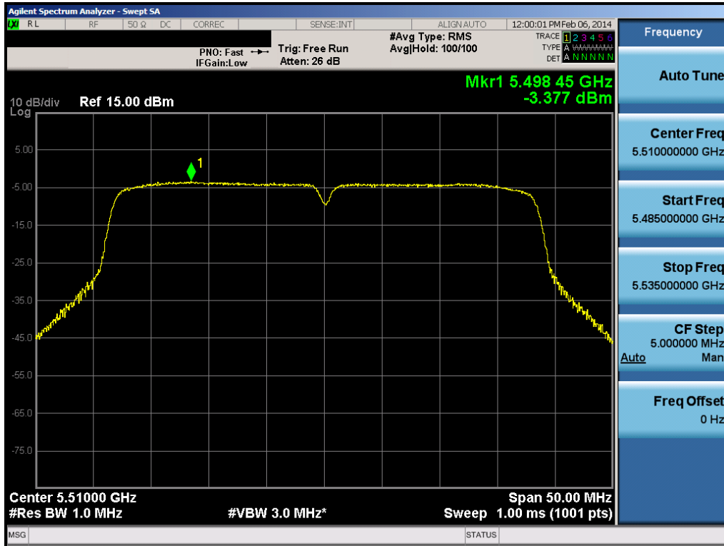
Plot 6-57. Peak Power Spectral Density Plot (40MHz BW 802.11n (UNII Band 2C) – Ch. 102)
