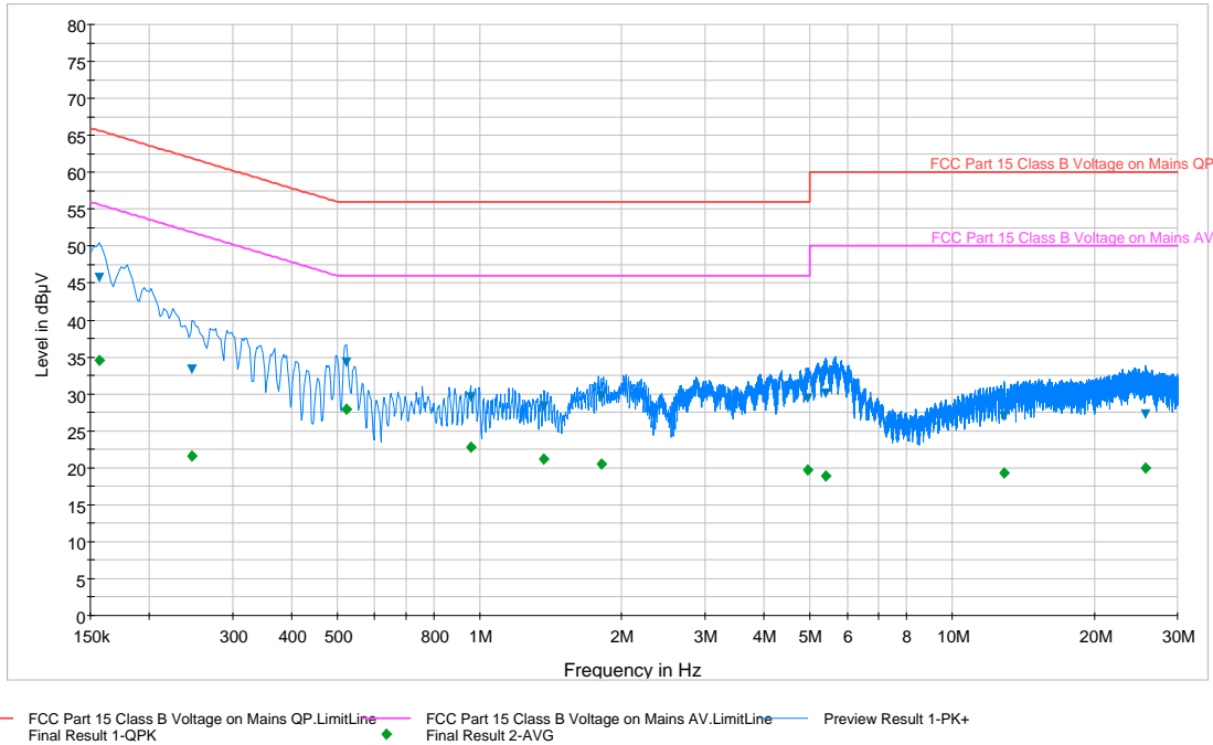
Plot 6-87. Line Conducted Plot with 802.11a UNII Band 2A (L1)
