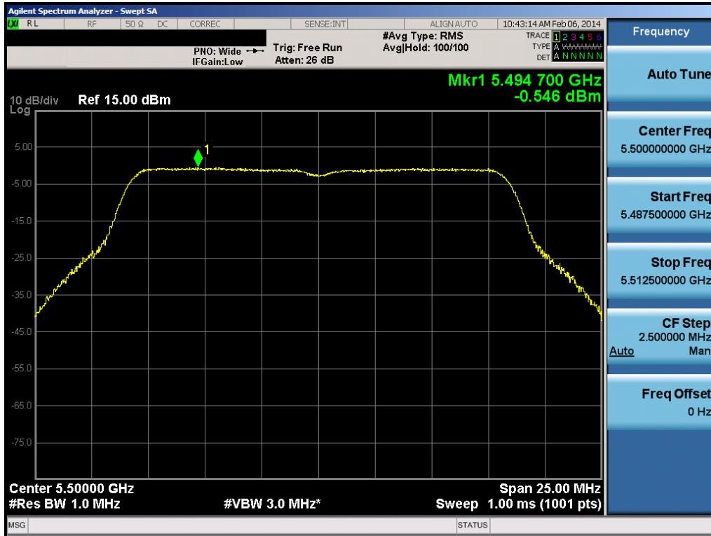
Plot 6-51. Peak Power Spectral Density Plot (802.11a (UNII Band 2C) – Ch. 100)
