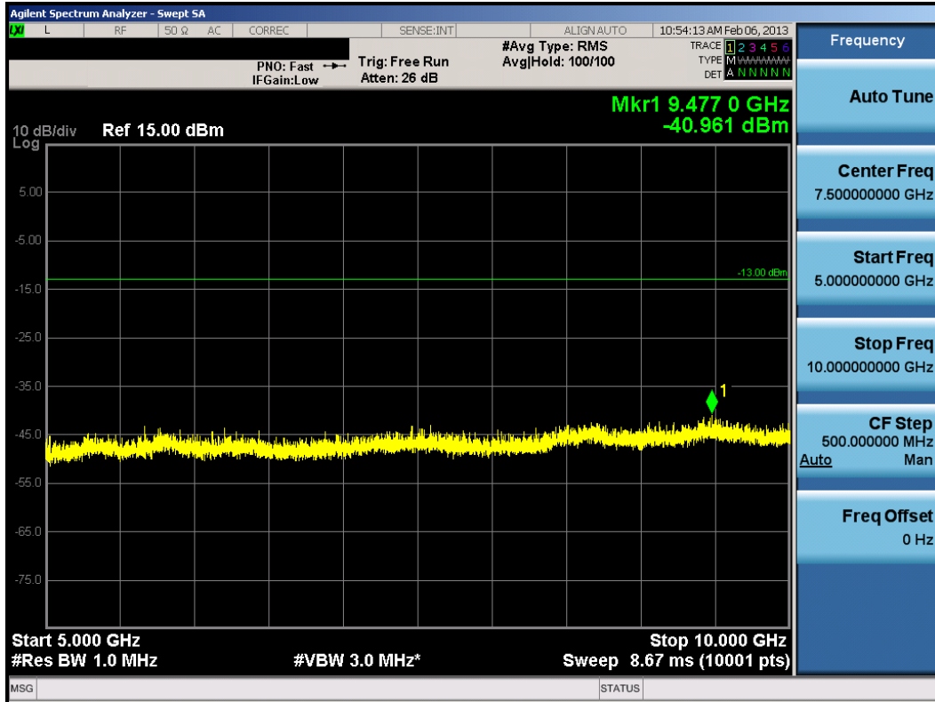
Plot 7-24. Conducted Spurious Plot (10.0MHz QPSK – RB Size 1, RB Offset 0 – Mid Channel)
