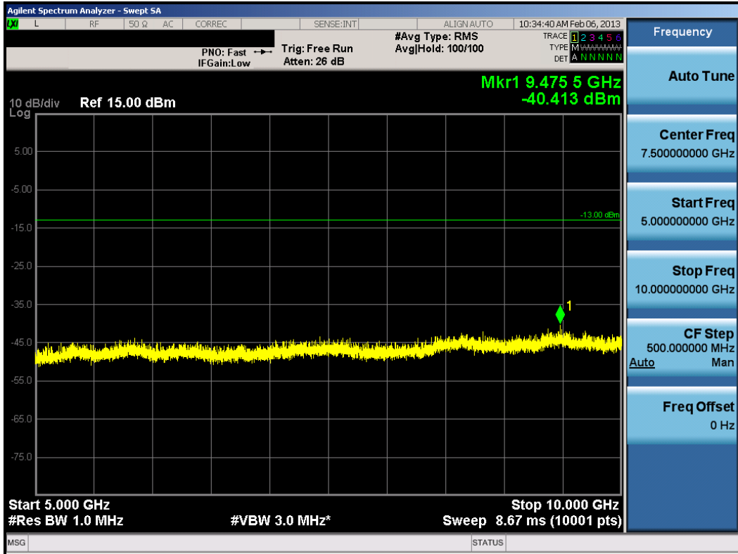
Plot 7-10. Conducted Spurious Plot (5.0MHz QPSK – RB Size 1, RB Offset 0 – Mid Channel)
