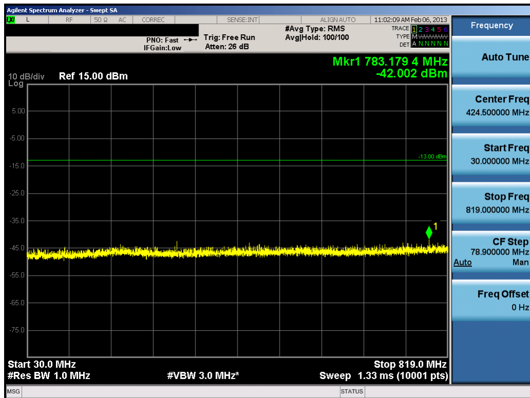
Plot 7-25. Conducted Spurious Plot (10.0MHz QPSK – RB Size 1, RB Offset 0 – High Channel)
