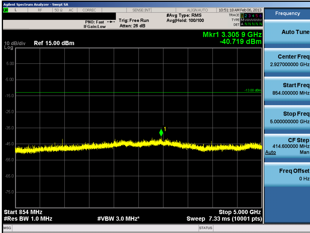
Plot 7-20. Conducted Spurious Plot (10.0MHz QPSK – RB Size 1, RB Offset 0 – Low Channel)
