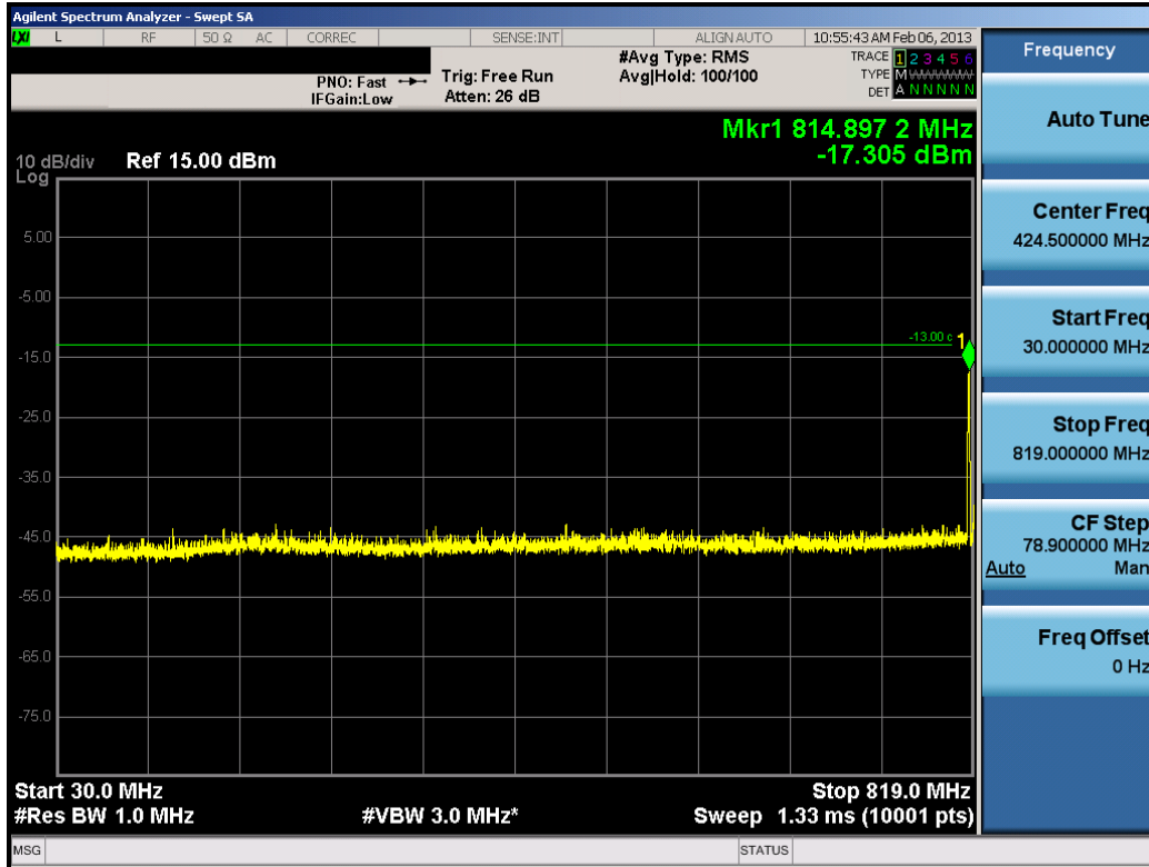
Plot 7-22. Conducted Spurious Plot (10.0MHz QPSK – RB Size 1, RB Offset 0 – Mid Channel)
