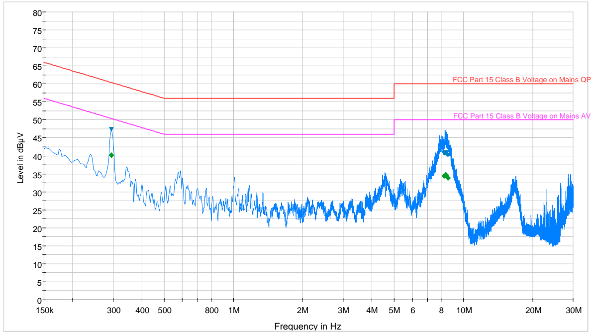
Plot 6-86. Line Conducted Plot with 802.11a UNII Band 2 (N)
