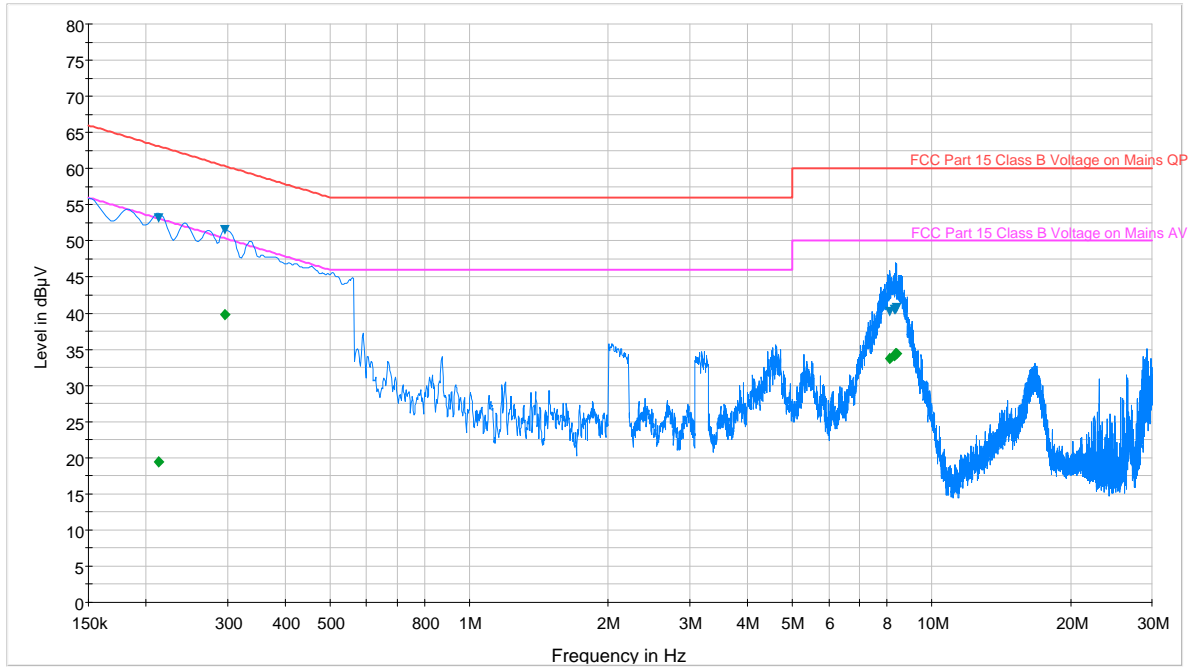
Plot 6-88. Line Conducted Plot with 802.11a UNII Band 3 (N)
