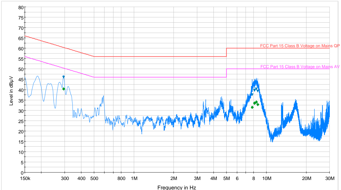
Plot 6-84. Line Conducted Plot with 802.11a UNII Band 1 (N)
