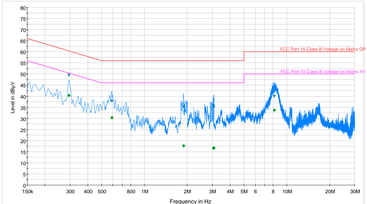
Plot 6-85. Line Conducted Plot with 802.11a UNII Band 2 (L1)
