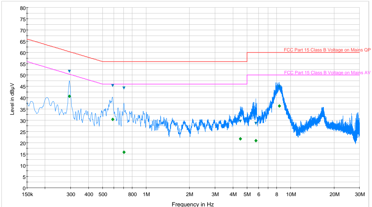
Plot 6-83. Line Conducted Plot with 802.11a UNII Band 1 (L1)
