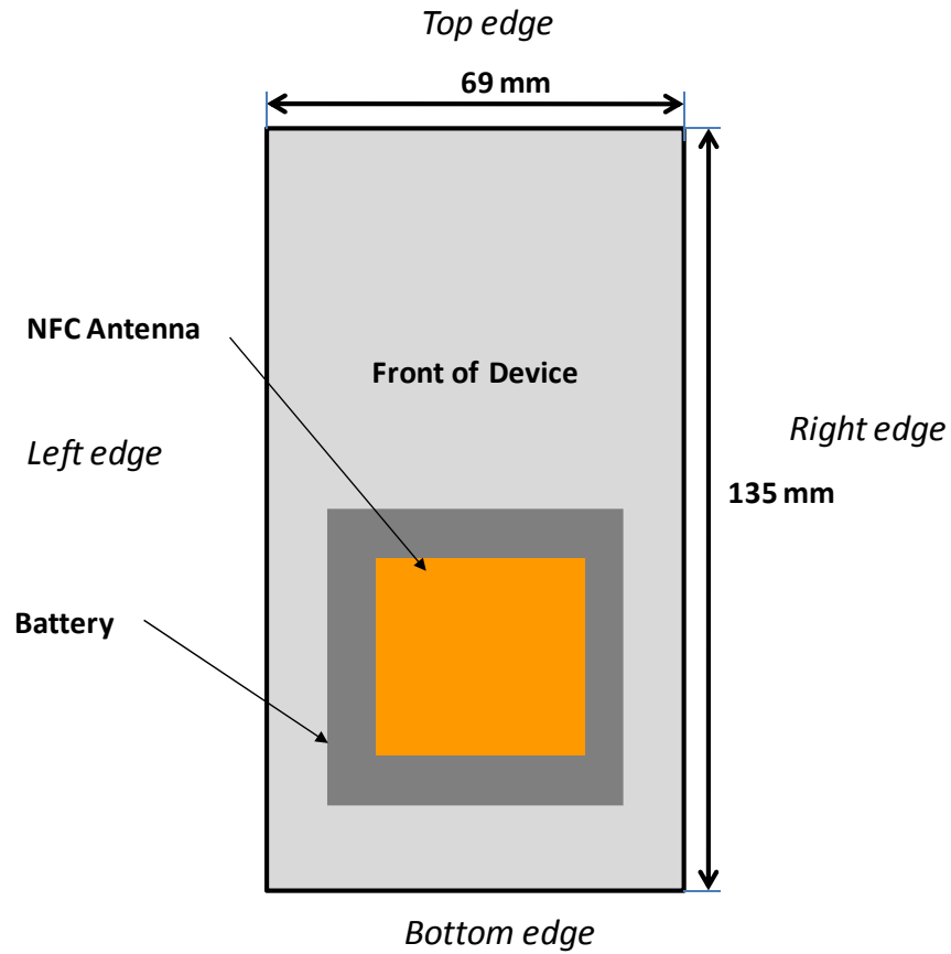
Figure 1-2 NFC Antenna Locations
