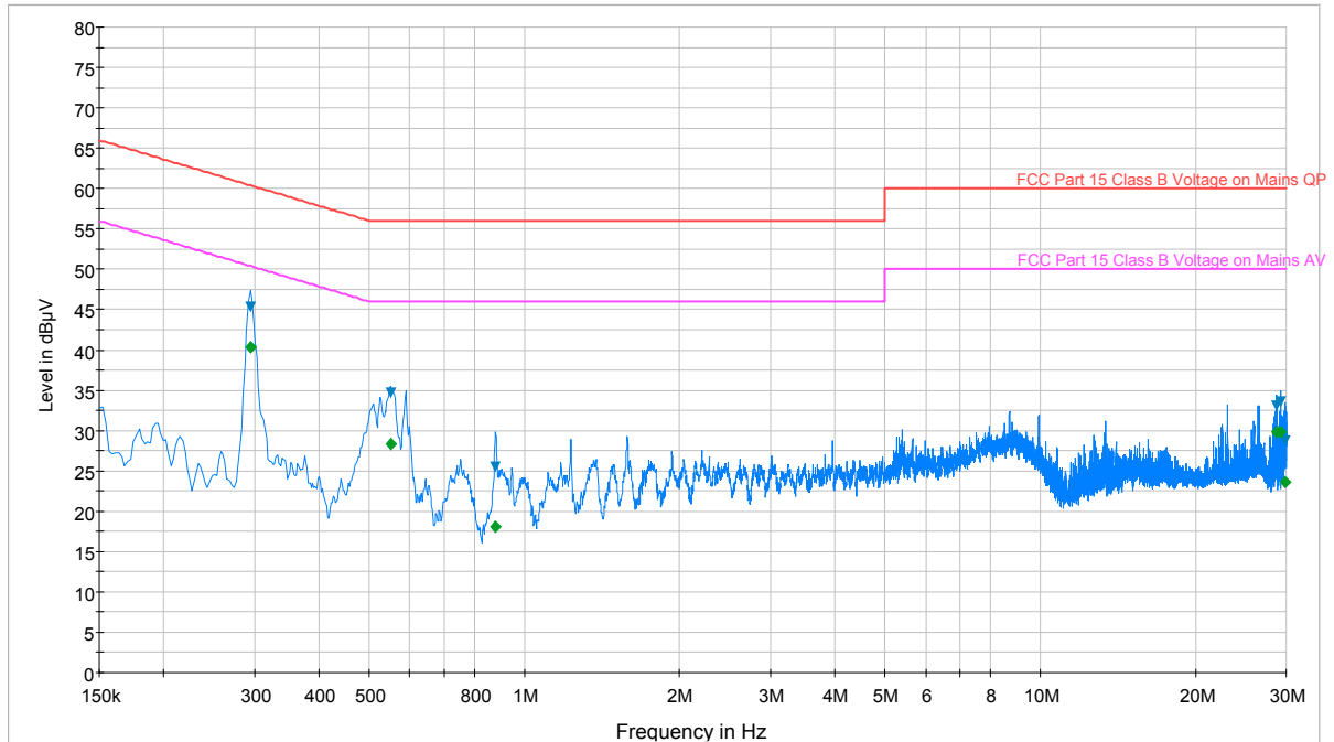
Plot 6-17. Line Conducted Plot with Bluetooth LE (L1)
