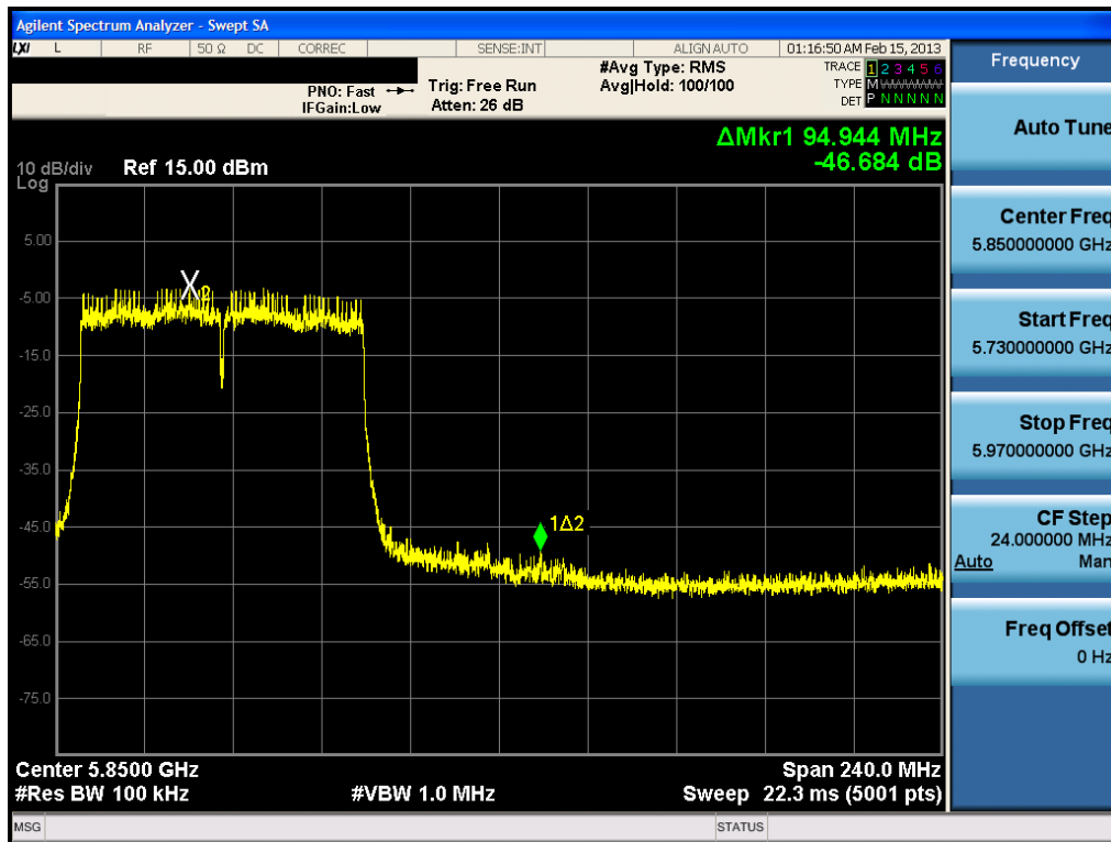
Plot 6-50. Upper Band Edge Plot (80MHz BW 802.11ac (5.8GHz) – Ch. 155)
