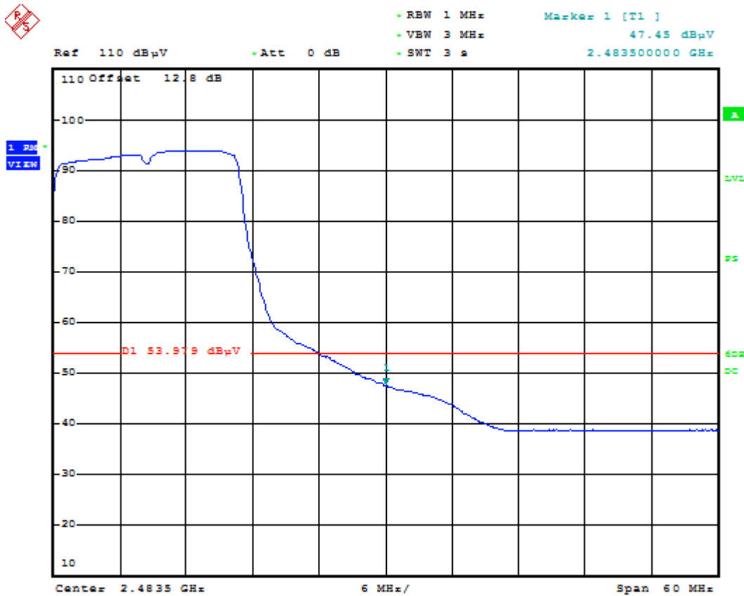
Plot 6-65. Radiated Restricted Upper Band Edge Measurement (Average)
