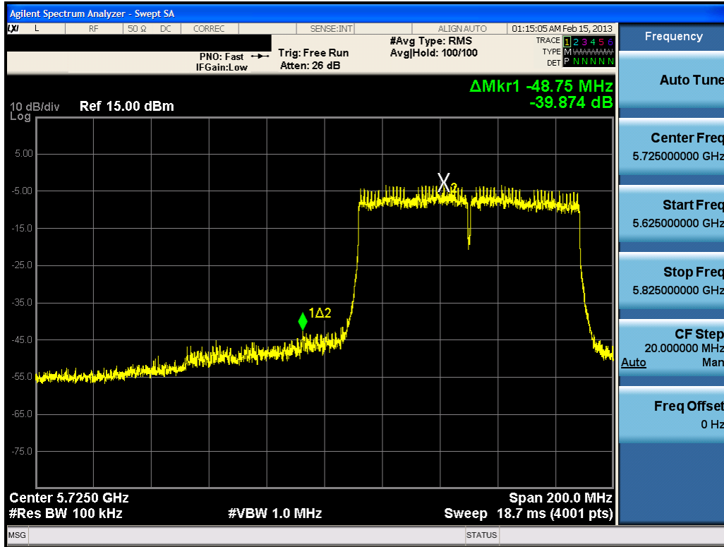
Plot 6-49. Lower Band Edge Plot (80MHz BW 802.11ac (5.8GHz) – Ch. 155)
