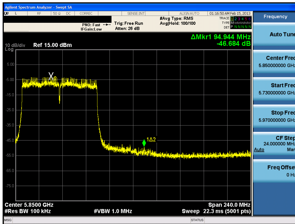
Plot 6-50. Upper Band Edge Plot (80MHz BW 802.11ac (5.8GHz) – Ch. 155)
