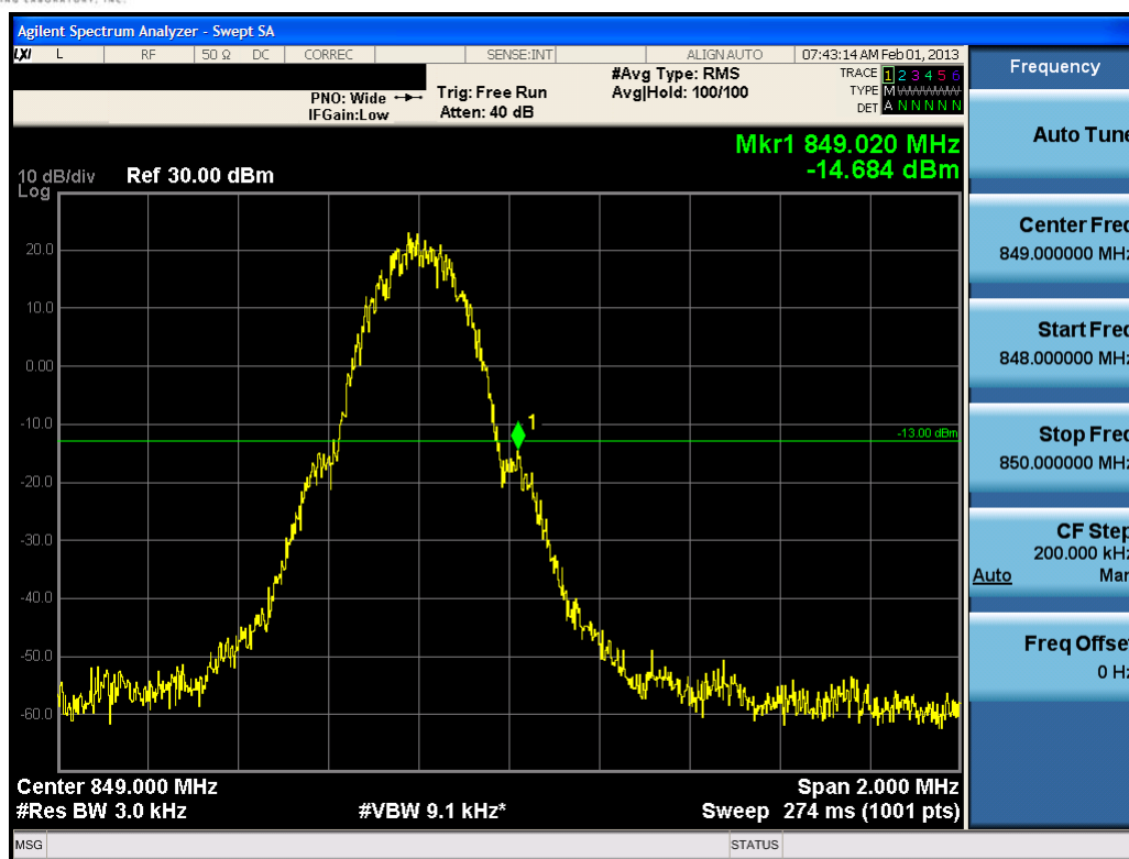
Plot 7-9. Band Edge Plot (Cellular GSM Mode – Ch. 251)
