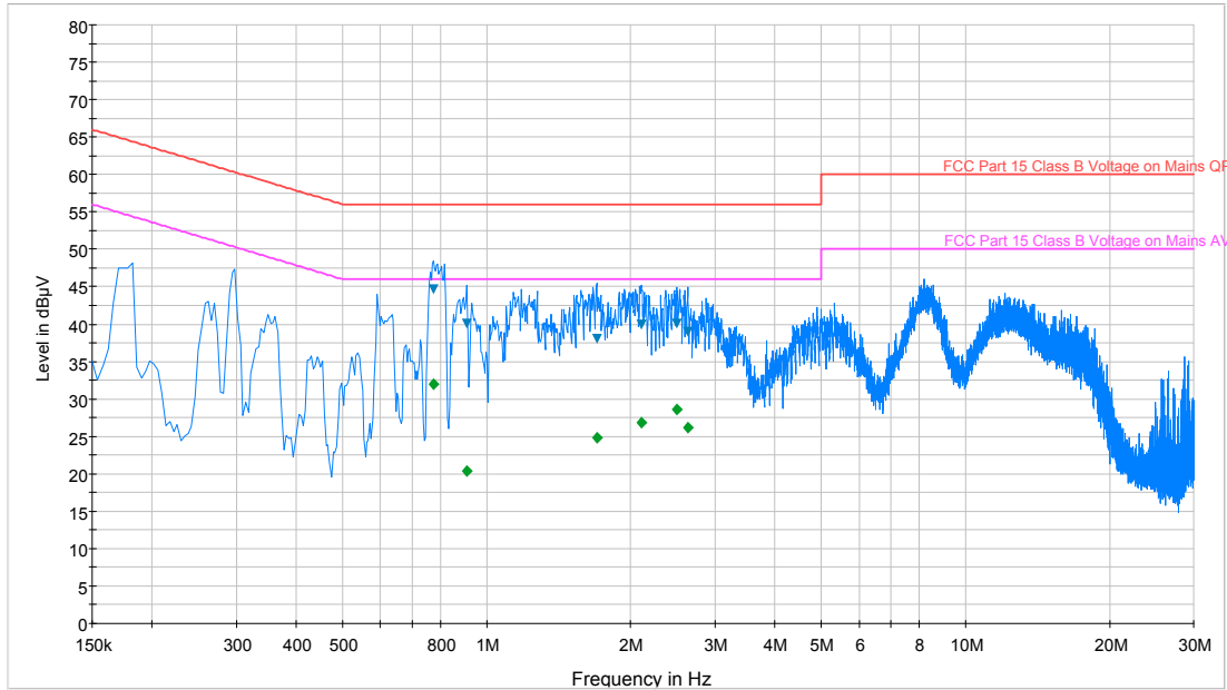
Plot 6-20. Line Conducted Plot with Bluetooth LE (N)
