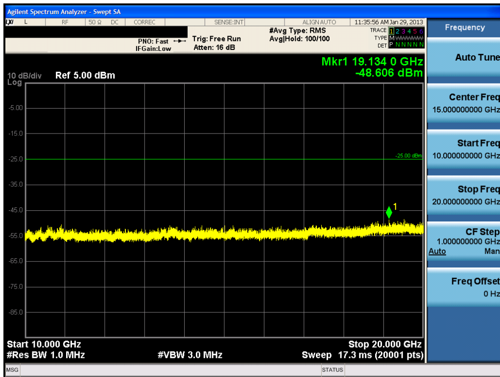
Plot 6-62. Conducted Spurious Plot (802.11a – Ch. 157)
