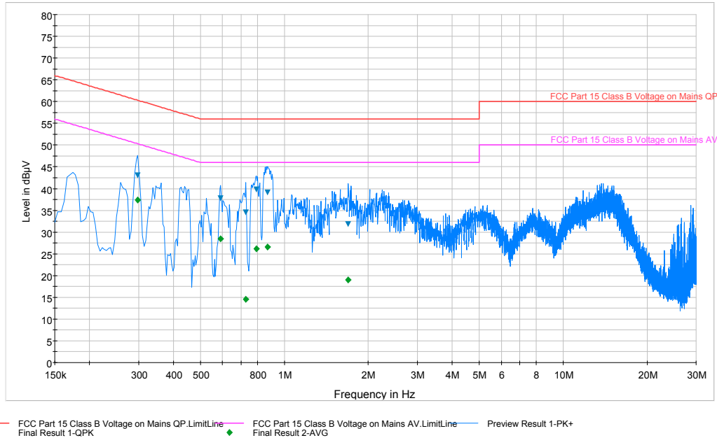
Plot 6-73. Line Conducted Plot with 802.11b (L1)
