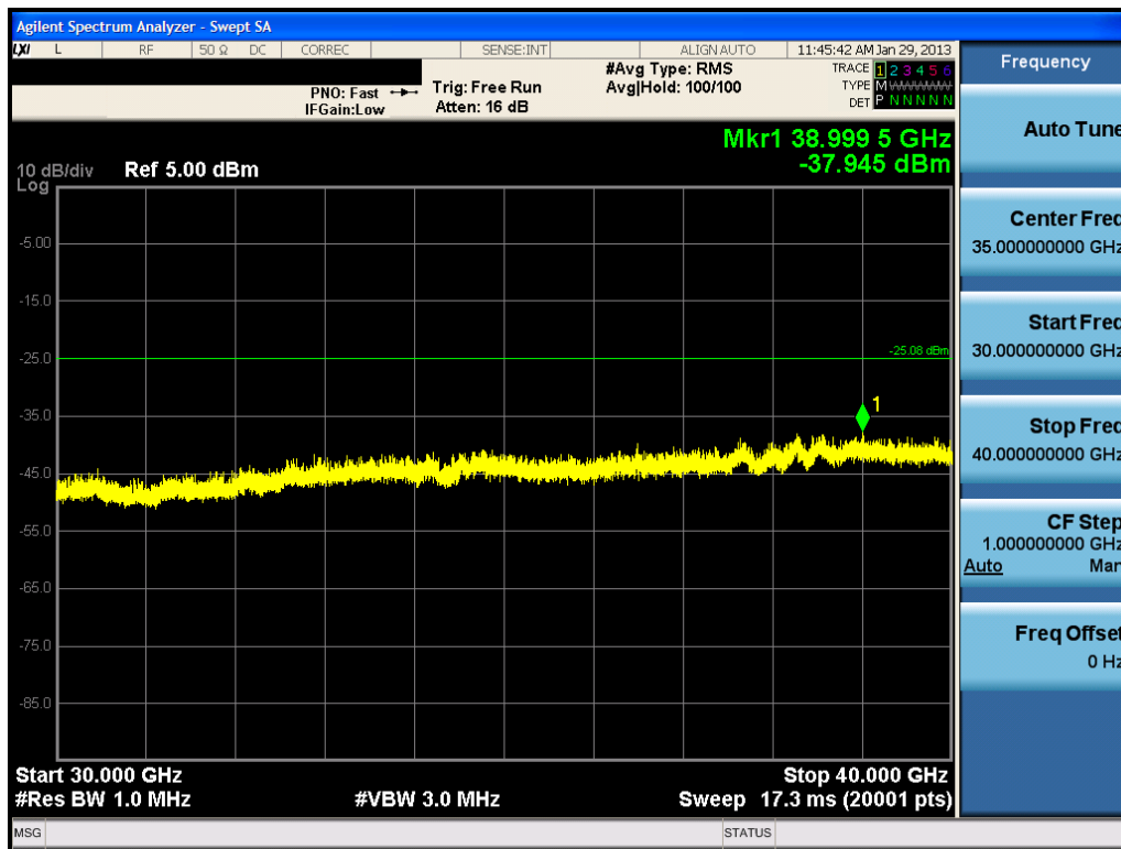
Plot 6-68. Conducted Spurious Plot (802.11a – Ch. 165)
