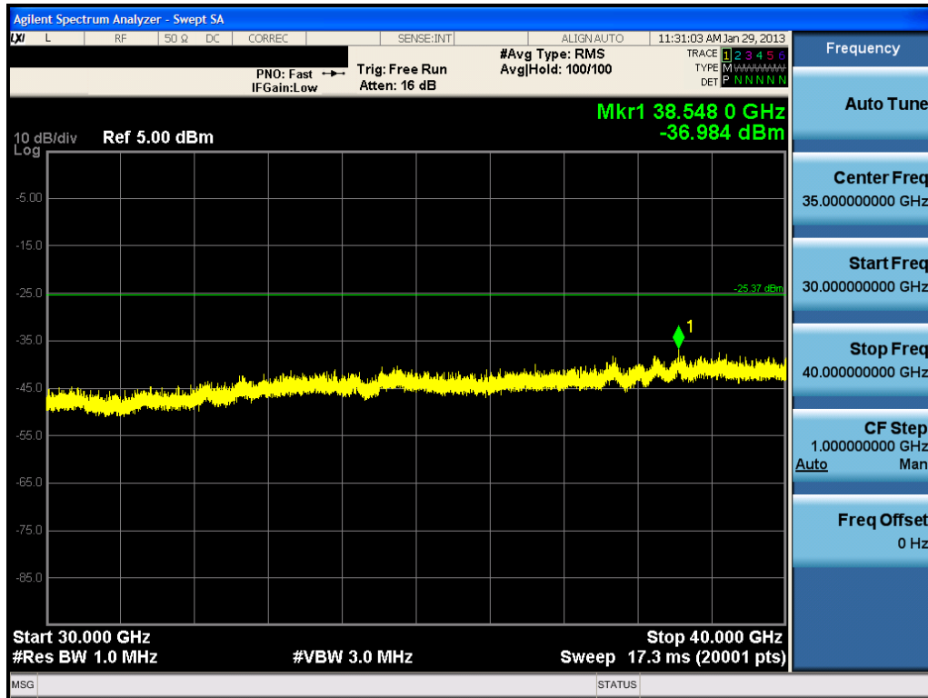
Plot 6-60. Conducted Spurious Plot (802.11a – Ch. 149)
