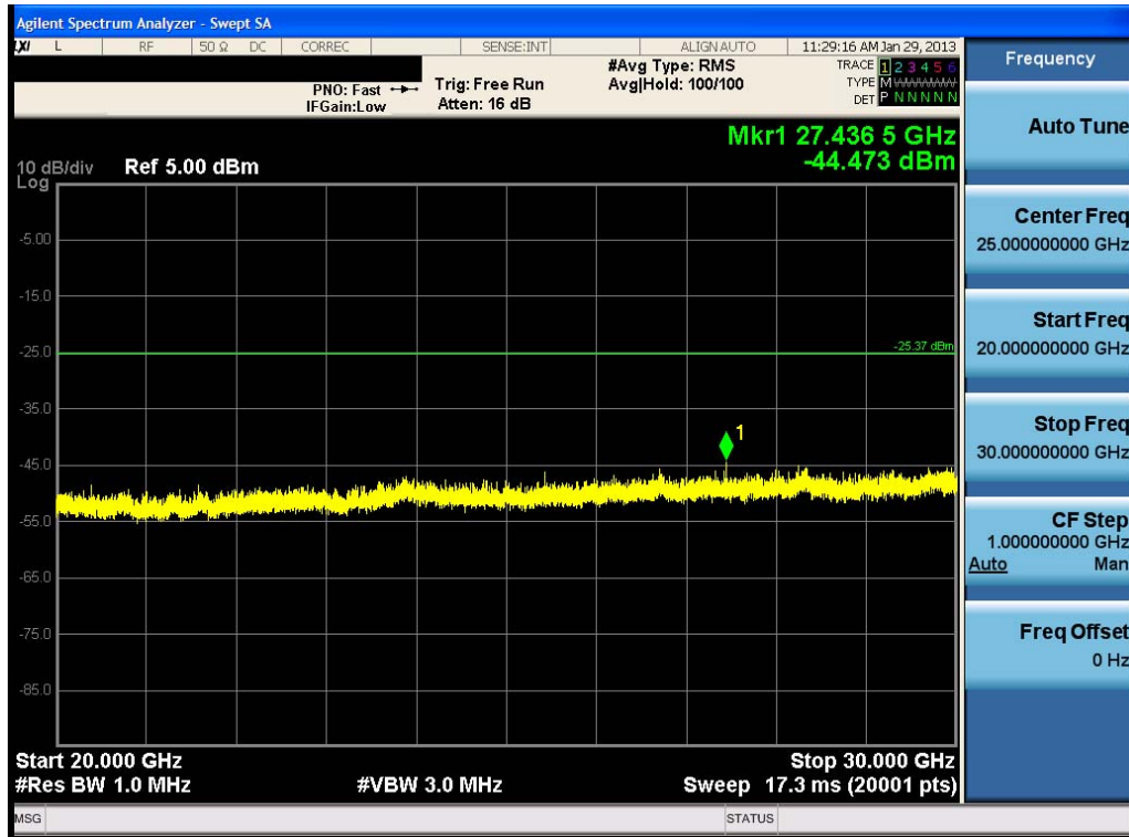
Plot 6-59. Conducted Spurious Plot (802.11a – Ch. 149)
