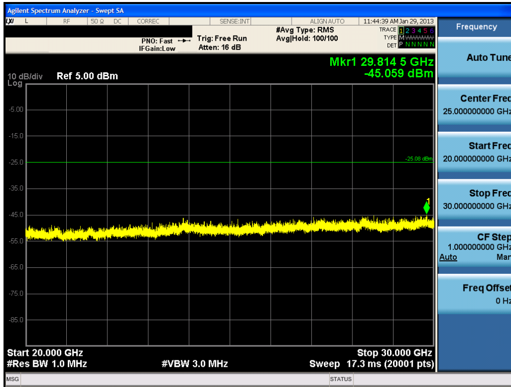
Plot 6-67. Conducted Spurious Plot (802.11a – Ch. 165)
