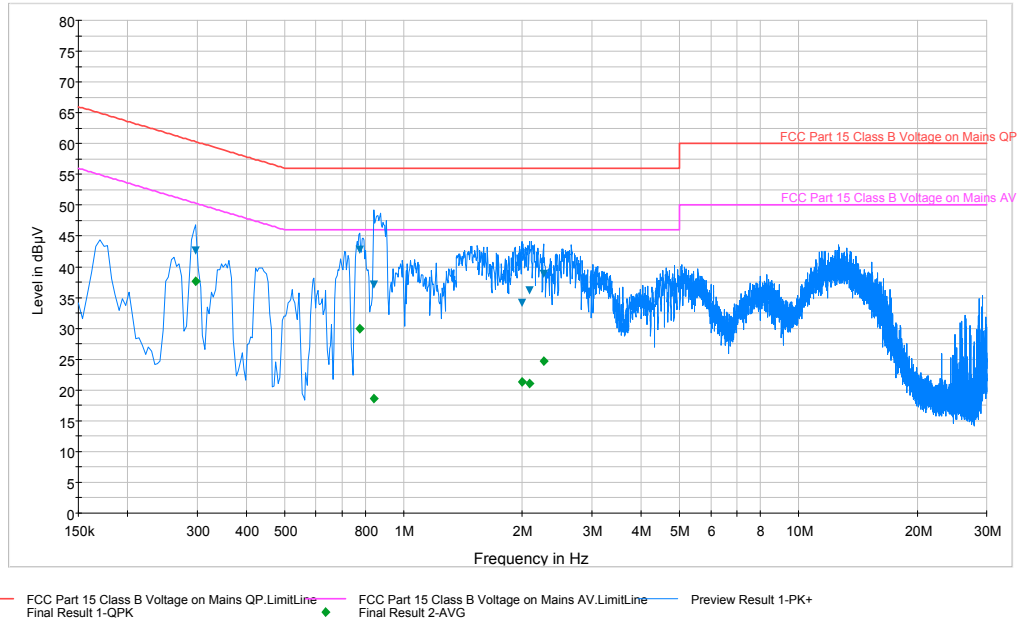
Plot 6-74. Line Conducted Plot with 802.11b (N)
