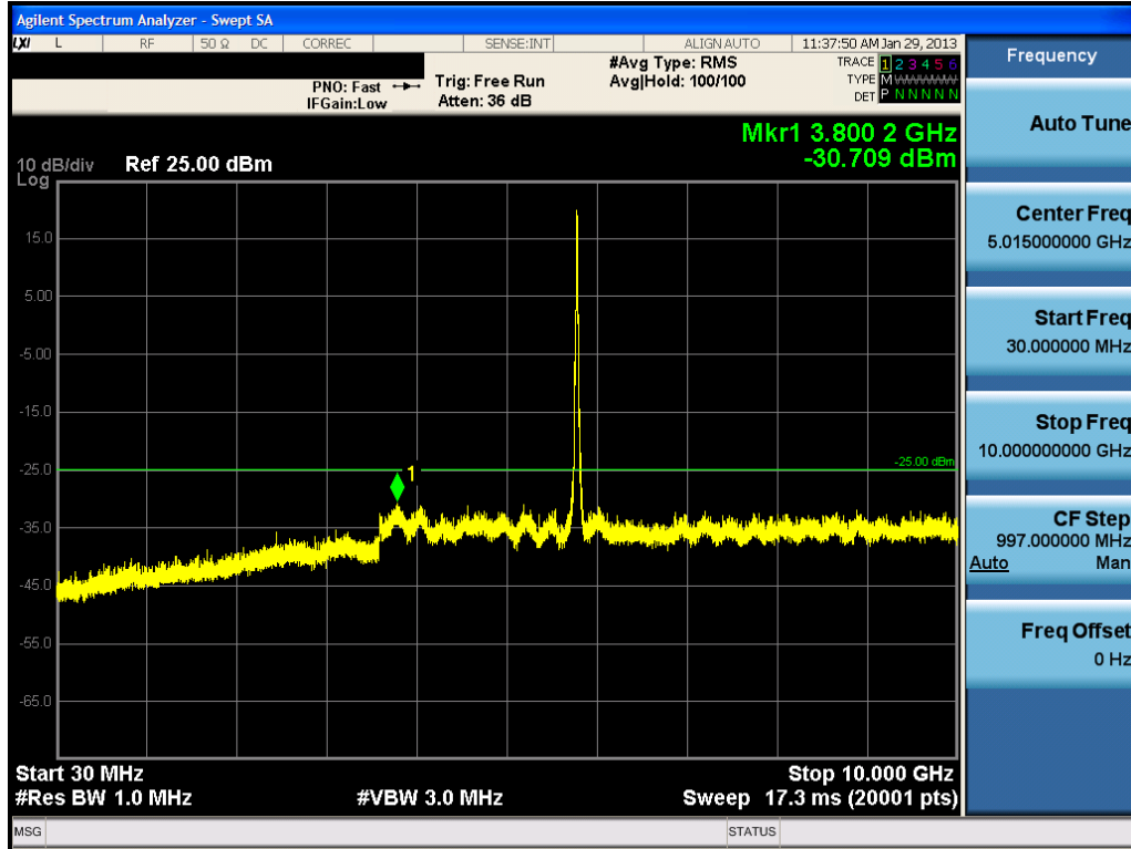
Plot 6-61. Conducted Spurious Plot (802.11a – Ch. 157)
