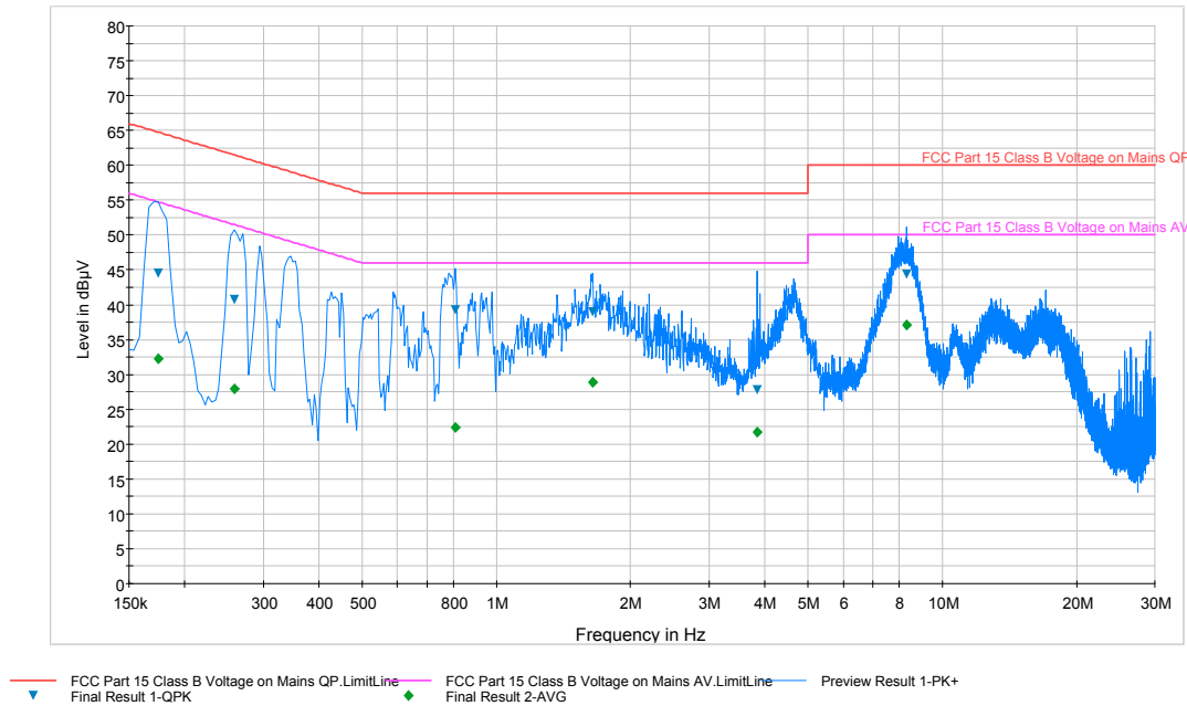
Plot 6-75. Line Conducted Plot with 802.11a (L1)
