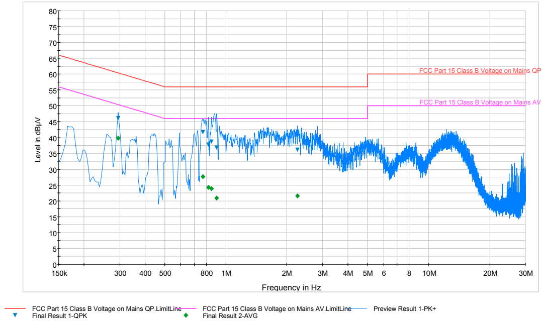
Plot 6-76. Line Conducted Plot with 802.11a (N)
